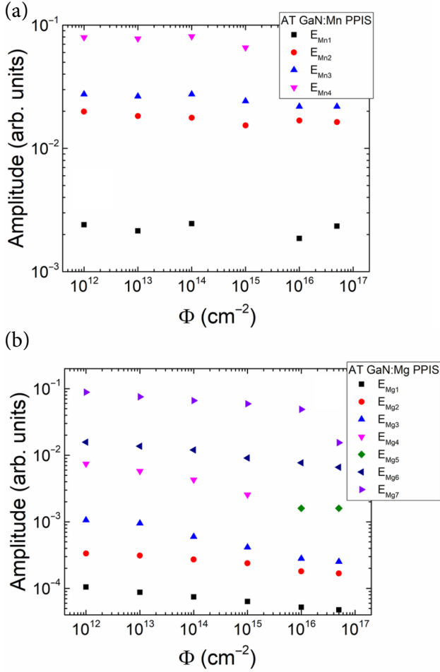
Fig. 2. (Coloured online.) Amplitudes of the PPI spectrum components, proportional to the initial filling of different traps, estimated from fitted PPI spectra for the pristine and neutron-irradiated samples (AT GaN:Mn (a) and AT GaN:Mg (b)), as functions of neutron irradiation fluence.
