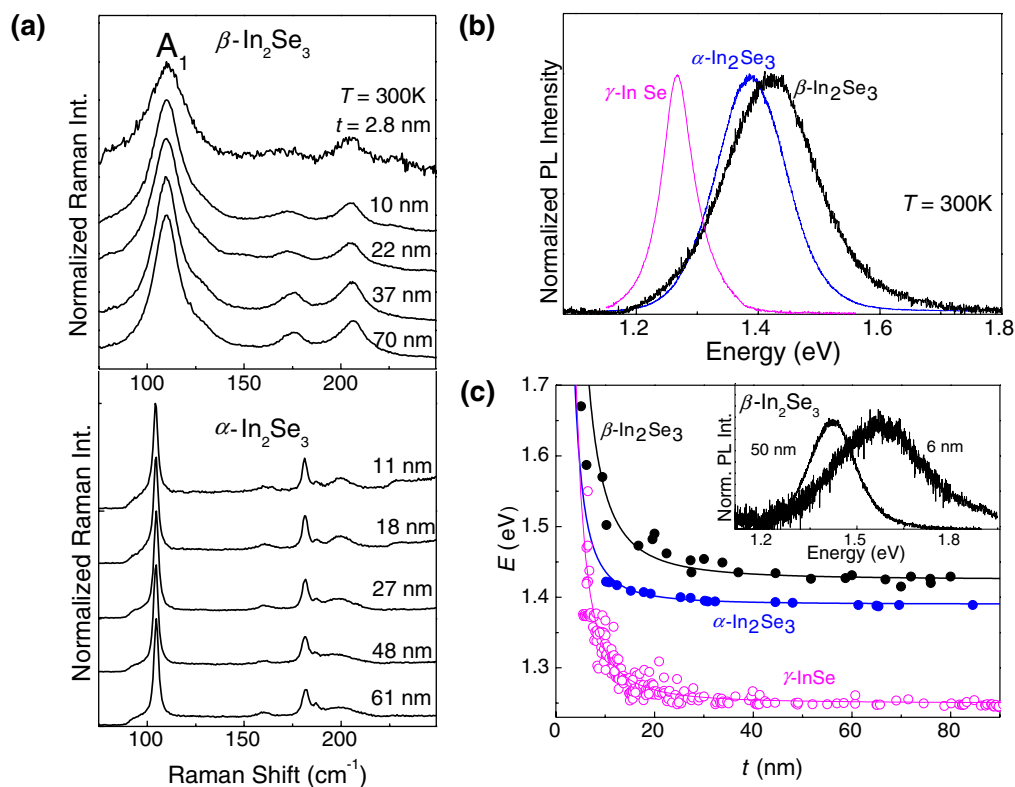
Figure VII.15. (a) Normalized Raman spectra of as-grown \beta - \text{In}_2\text{Se}_3 layers (top) and exfoliated flakes of \alpha - \text{In}_2\text{Se}_3 (bottom) at T = 300 K ( P = 0.1 mW and \lambda = 633 nm). (b) Normalized \mu\text{PL} spectra of bulk \gamma -InSe, \beta - \text{In}_2\text{Se}_3 and \alpha - \text{In}_2\text{Se}_3 at T = 300 K ( \lambda = 633 nm and P = 0.1 mW). (c) Measured and calculated dependence of the peak energy, E , of the PL emission on layer thickness t of as-grown \beta - \text{In}_2\text{Se}_3 (black dots) and exfoliated Bridgman-grown \alpha - \text{In}_2\text{Se}_3 (blue dots) and \gamma -InSe (magenta dots) flakes. Inset: Normalized PL spectra of \beta - \text{In}_2\text{Se}_3 with t \sim 50 nm and 6 nm at T = 300 K. Adapted from [1117], © IOP Publishing Ltd.
