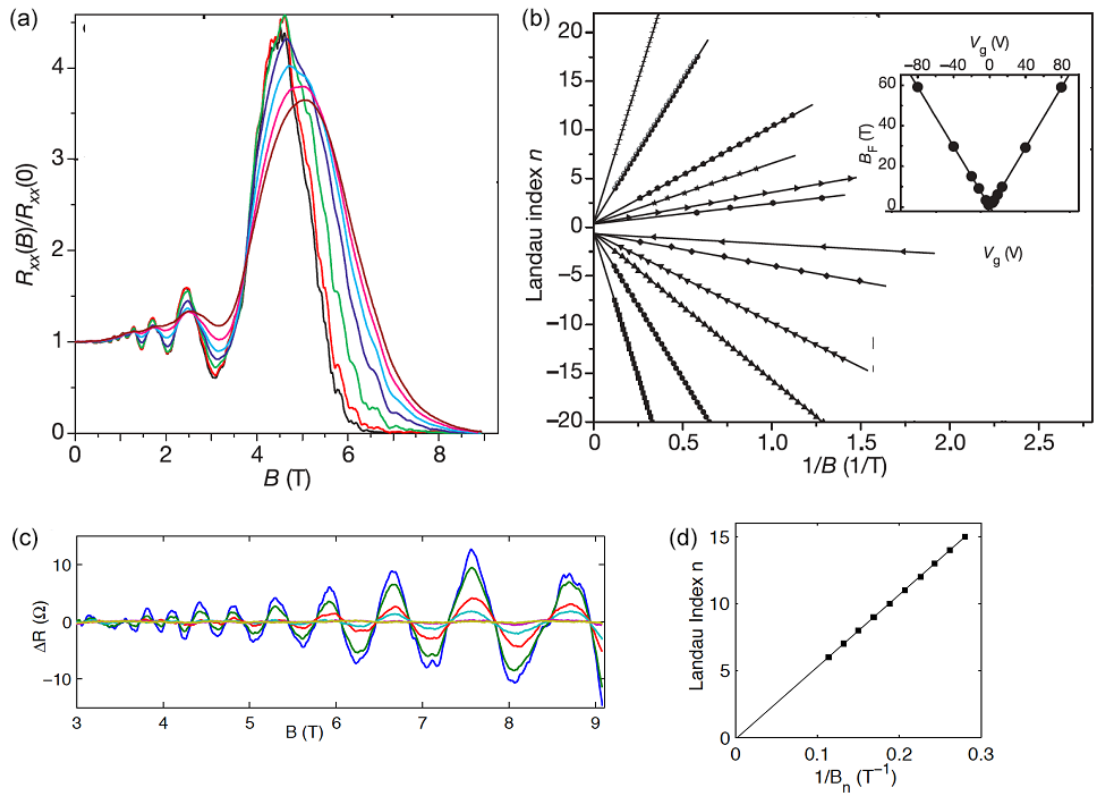
Figure IX.58. Shubnikov–de Haas oscillations of the magnetoresistance in (a) and (b) SLG on \text{SiO}_2 [1617] and (c), (d) MLG on 4H-SiC(000–1) (C-face) [1620] for different T from 4 to 70 K. (b) The minima in \rho_{xx} are plotted as a function of 1/B (so called fan plots) to determine the charge density at a particular gate voltage. (d) Same analysis for the data in (c), but plotting the maxima in \rho_{xx} .
