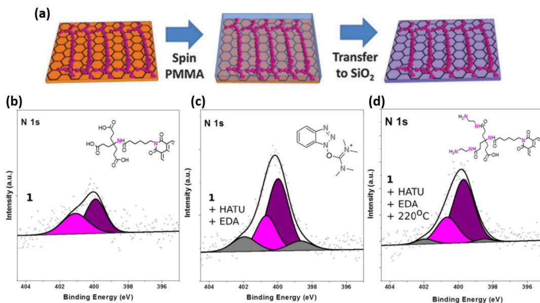
Figure VIII.9. (a) Schematic FLAT, in which perylene functionalized graphene is transferred b-d) XPS spectra of perylene on CVD-SLG for each derivitization step. (b) As-transferred perylene 1 on SLG. Inset: Partial structure of perylene 1 with corresponding nitrogen contributions. (c) Perylene 1 on SLG after reaction with HATU and EDA. The two new contributions are from HATU residue. Inset: Chemical structure of HATU. (d) After annealing of derivatized sample at 220 °C. The HATU contributions reduce, but the amine signal increases. Inset: Partial structure of perylene 1 after reaction, depicting corresponding nitrogen contributions. Adapted from [1327] with permission of The Royal Society of Chemistry.
