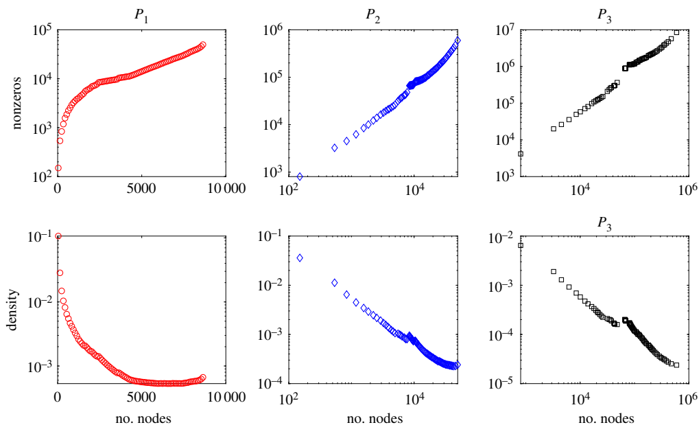
Figure 4. Evolution of number of nonzeros and of the density of the matrices P_1 = A , P_2 , and P_3 associated with subgraphs of the largest connected component of the network CA-HEP. (Online version in colour.)
