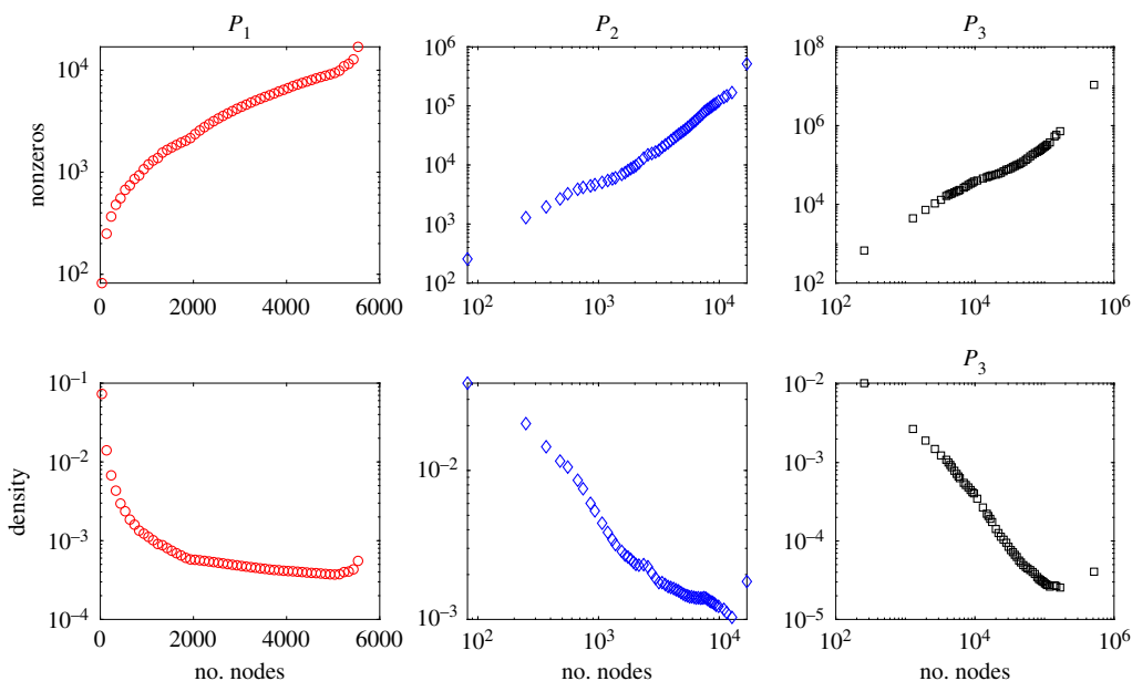
Figure 5. Evolution of number of nonzeros and of the density of the matrices P_1 = A , P_2 , and P_3 associated with subgraphs of the largest connected component of the network ERDOS02. (Online version in colour.)
