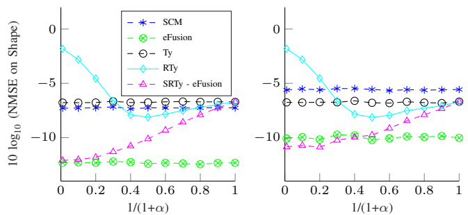
Fig. 3. NMSE on shape matrix versus 1/(1+\alpha) in the spiked covariance model for p = 12 , n = 20 , where the data is close to Gaussian ( d = 20 , left) and heavy-tailed ( d = 3 , right).
