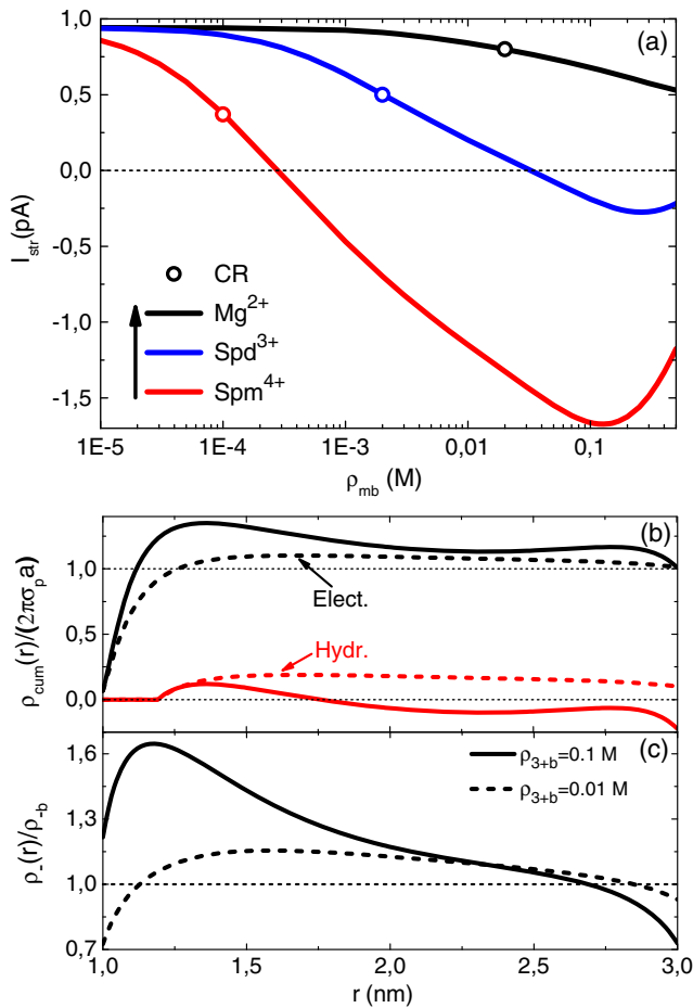
FIG. 2 (color online). (a) Streaming current curves at the pressure gradient \Delta P_z = 1 bar against the reservoir density of the multivalent counterion species given in the legend. Open circles mark the charge reversal (CR) points. (b) Electrostatic (black curves) and hydrodynamic (red curves) cumulative charge densities, and (c) \text{Cl}^- densities in the \text{KCl} + \text{SpdCl}_3 liquid at the reservoir concentrations \rho_{3+b} = 0.01 M (dashed curves) and 0.1 M (solid curves). The neutral nanopore ( \sigma_m = 0 ) contains a ds DNA of charge density \sigma_p = 0.4 e/nm 2 , with the bulk \text{K}^+ density \rho_{+b} = 0.1 M in all figures.
