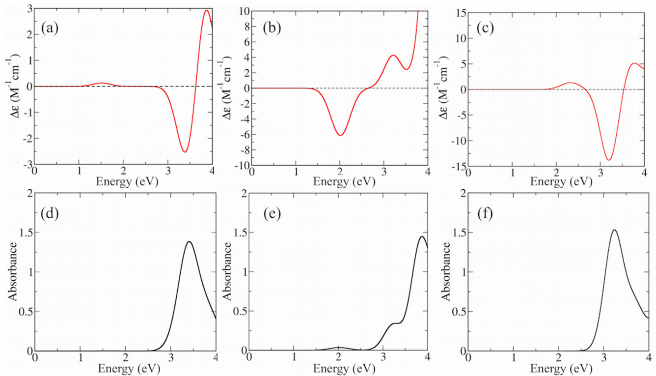
FIG. 6. (a)–(c) Calculated average CD of \text{Ag}_4 , \text{Ag}_5^{+1} , and \text{Ag}_6^{+2} ; (d)–(f) the calculated average optical spectra of \text{Ag}_4 , \text{Ag}_5^{+1} , and \text{Ag}_6^{+2} .
