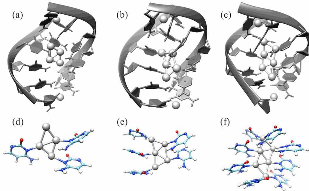
FIG. 2. (a)–(c) Structure of the \text{Ag}_4^0\text{@C}_6\text{-[Ag}^+ \text{]}_2\text{-C}_6 , \text{Ag}_5^{+1}\text{@C}_6\text{-[Ag}^+ \text{]}_2\text{-C}_6 , and \text{Ag}_6^{+2}\text{@C}_6\text{-[Ag}^+ \text{]}_2\text{-C}_6 ; (d)–(f) the Ag core and their neighbor atoms in the Ag:DNAs, respectively.
