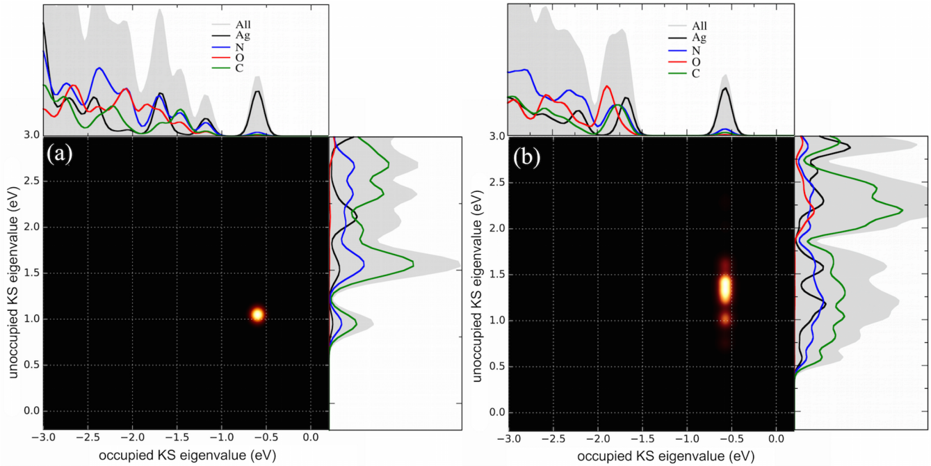
FIG. 5. (a) Transition contribution map of the \text{Ag}_5^{+1}@\text{C}_6-[\text{Ag}^+]_2-\text{C}_6 at 1.7 eV and (b) the transition contribution map of the \text{Ag}_6^{+2}@\text{C}_6-[\text{Ag}^+]_2-\text{C}_6 at 2.0 eV. The horizontal PDOS are for the occupied states, while the vertical PDOS are for the unoccupied states in the Ag:DNAs.
