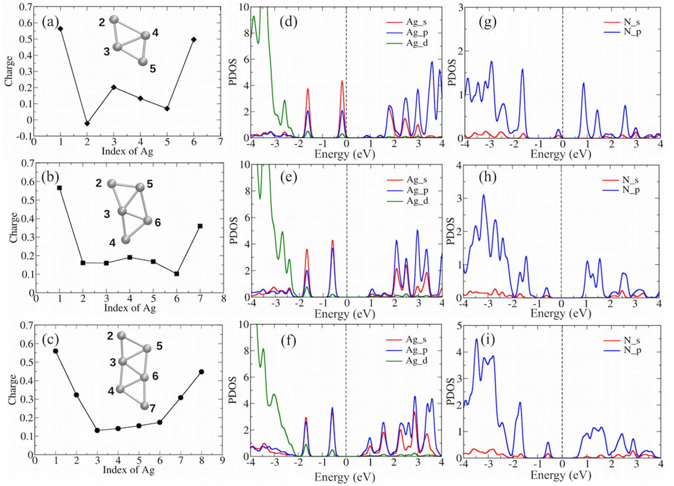
FIG. 4. (a)–(c) Bader charges of the Ag atoms in the \text{Ag}_4^0@C_6-[\text{Ag}^+]_2-C_6 , \text{Ag}_5^{+1}@C_6-[\text{Ag}^+]_2-C_6 , and \text{Ag}_6^{+2}@C_6-[\text{Ag}^+]_2-C_6 . The top Ag atom was marked by 1 and the bottom Ag was marked by 6 , 7 , and 8 , respectively. The labeling of the Ag core atoms can be seen in the inset of the figures. (d)–(f) The PDOS of the core Ag atoms and (g)–(i) the PDOS of their neighbor N atoms in the \text{Ag}_4^0@C_6-[\text{Ag}^+]_2-C_6 , \text{Ag}_5^{+1}@C_6-[\text{Ag}^+]_2-C_6 , and \text{Ag}_6^{+2}@C_6-[\text{Ag}^+]_2-C_6 .
