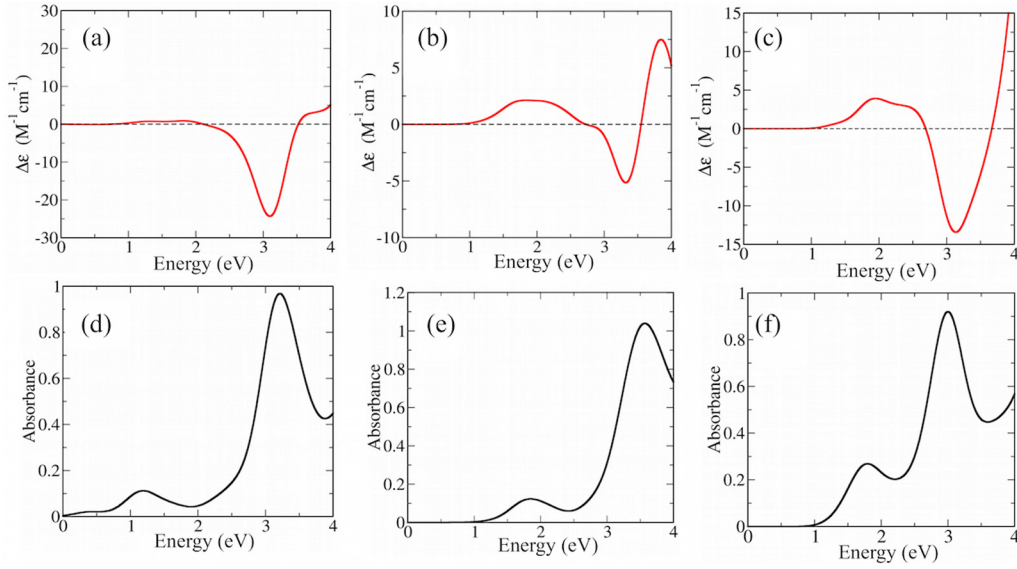
FIG. 3. (a)–(c) Calculated CD and (d)–(f) the calculated optical absorption spectra of the \text{Ag}_4^0\text{@C}_6\text{-[Ag}^+\text{]}_2\text{-C}_6 , \text{Ag}_5^{+1}\text{@C}_6\text{-[Ag}^+\text{]}_2\text{-C}_6 , and \text{Ag}_6^{+2}\text{@C}_6\text{-[Ag}^+\text{]}_2\text{-C}_6 .
