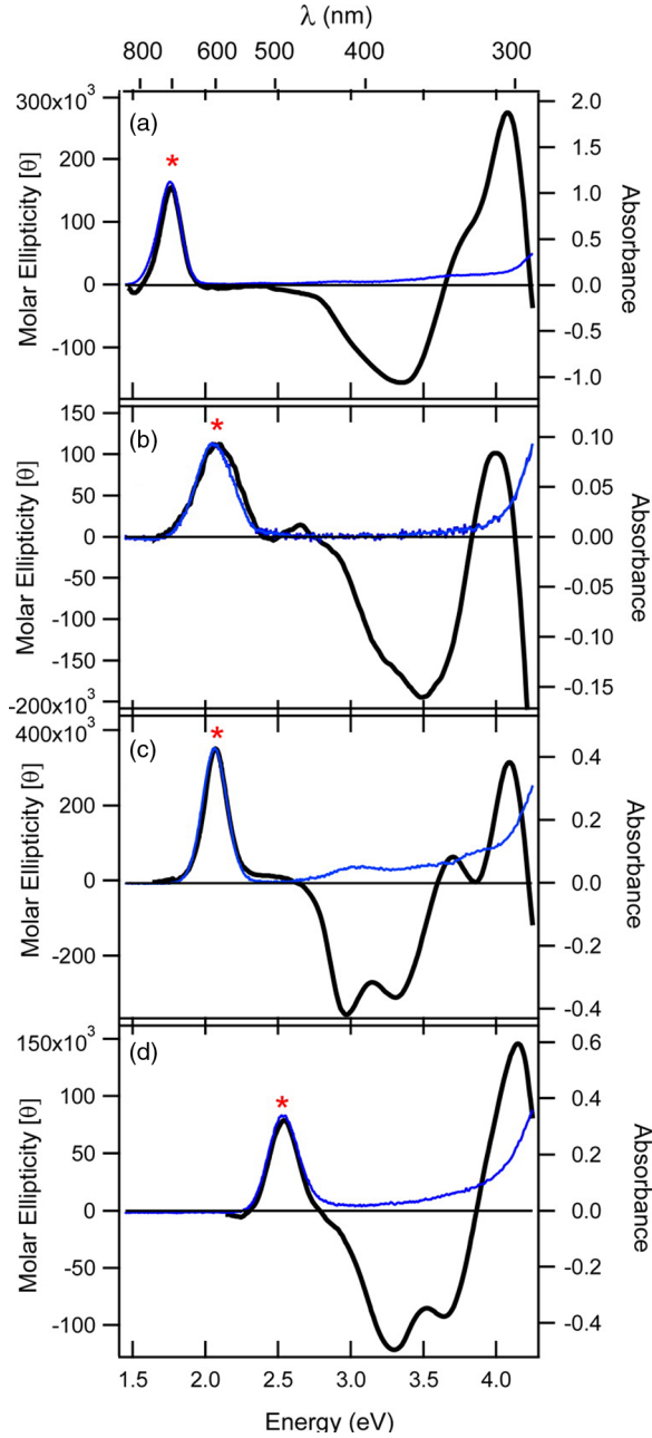
FIG. 1. CD (black) and absorption (blue) spectra of pure cluster solutions S1 (a), S2 (b), S3 (c) (aqueous solution), and S4 [(d); 50 MeOH]. A positive CD peak overlies the collective longitudinal cluster absorption peak (red stars). S1: CCCACCCAC-CCGCCCA, 12 \text{Ag}^0 , 8 or 9 \text{Ag}^+ ; S2: GGCAGGTTGGGGT-GACTAAAACCCCTTAATCCCC, 6 \text{Ag}^0 , 9 \text{Ag}^+ ; S3: CAC-CGCTTTTGCTTTTGGGGACGGATA, 6 or 7 \text{Ag}^0 , 8 or 9 \text{Ag}^+ ; S4: TGCCTTTTGGGGACGGATA, 4 \text{Ag}^0 , 6 \text{Ag}^+ . The figure is taken from [18] with permission.
