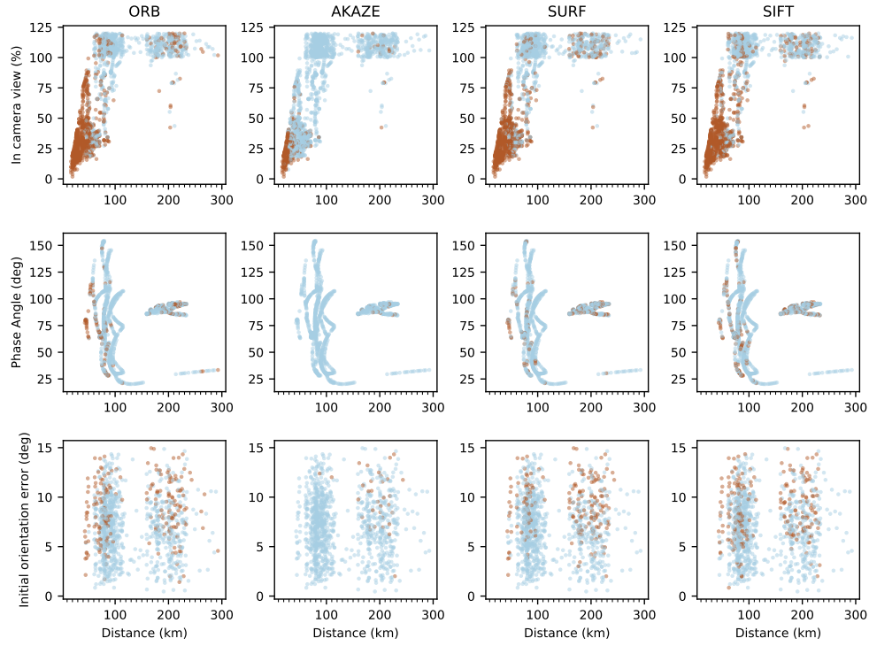
Figure 6. Successes (light blue) and failures (brown) in different situations based on real Rosetta NavCam images. This figure is produced the same way as 4, please refer to the image caption there.
