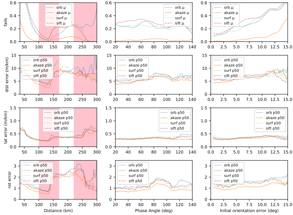
Figure 7. Failure rate and errors vs different situations based on real Rosetta NavCam images. Note how AKAZE (orange lines) has the lowest failure rate and lowest errors in almost all regions.
