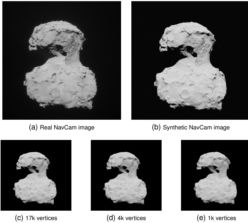
Figure 3. Five different image types were used in the study. Top left is an actual preprocessed Rosetta NavCam image, top right is an image rendered using a fitted Hapke reflectance model and a shape model with 1.9M vertices. Bottom row is rendered using a fitted lunar-Lambert reflectance model and shape models with varying vertex count: 17,000 (left), 4,000 (middle) and 1,000 (right).
