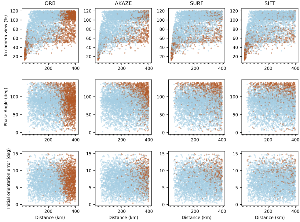
Figure 4. Successes (light blue) and failures (brown) of Monte Carlo samples with different feature extraction algorithms. For better sample separation when in-camera-view is exactly 100%, we add a 0–20% random component if the parameter value is 100%, so that values between 100–120% map to 100%.
