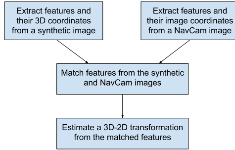
Figure 1. Overview of the algorithm analyzed in this work with its main steps visible.
