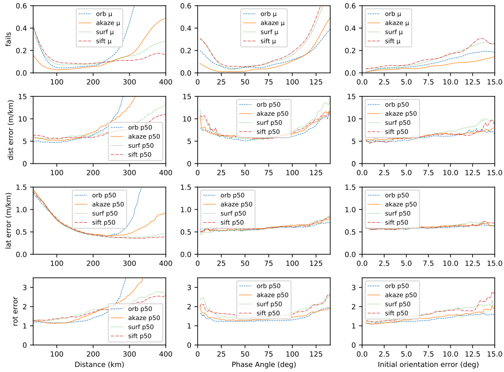
Figure 5. Failure rate and errors vs different situations.
