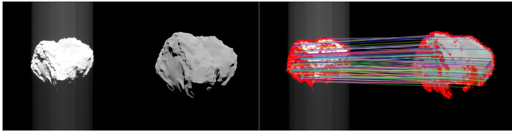
Figure 8. AKAZE features from overexposed NavCam image matched with features from onboard rendered 4,000 vertex shape model.
