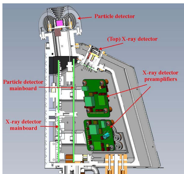
Fig. 5 Cross section of the SIXS sensor unit
