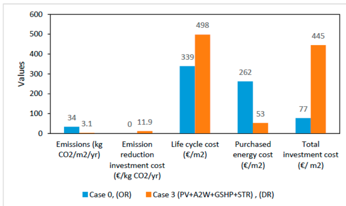
Figure 15. The emissions, emissions reduction cost, LCC, investment, and purchased energy cost comparison between Case 0 with OR buildings and Case 3 with DR buildings in the community.
