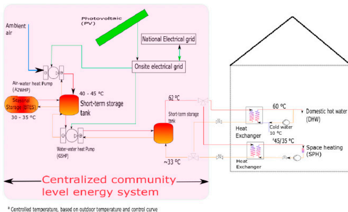
Figure 5. The schematic diagram of the centralized grid community-level district heating system for the old residential buildings based on PV, A2WHP, GSHP, and seasonal storage. (Case 3, PV + AW + GSHP + STR).
