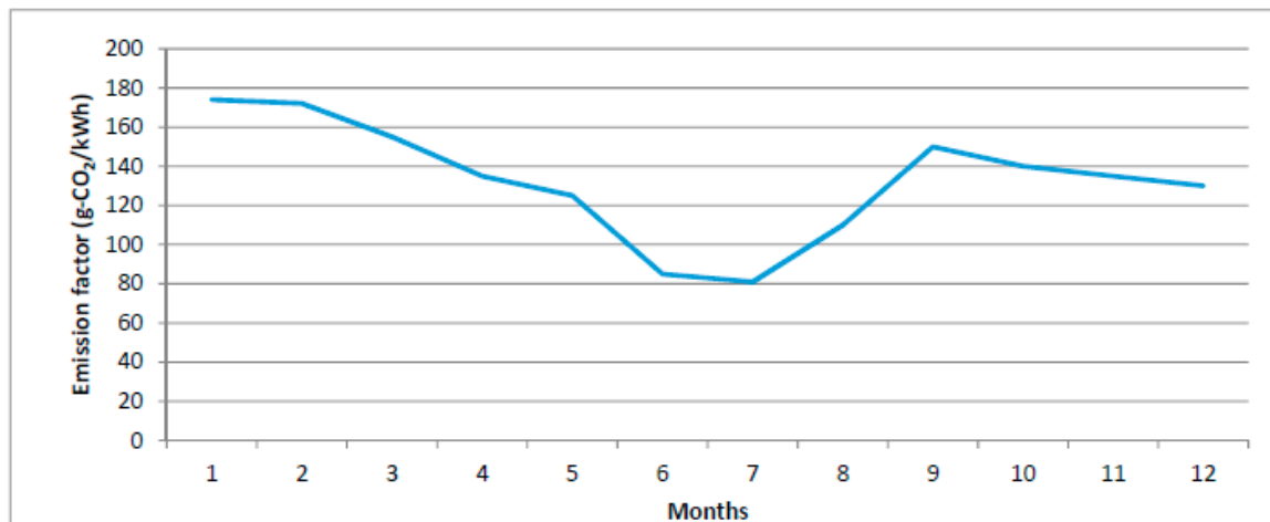
Figure 7. The average monthly emissions of the electrical grid of Finland [19,26].
