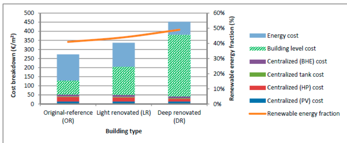
Figure 10. The breakdown of LCC of the old residential building community and centralized energy system based on PV and GSHP (Case 1, PV + GSHP).
