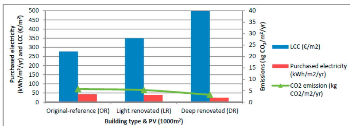
Figure 13. The annual purchased electricity, LCC, and CO 2 emissions from the centralized community-level PV, HP, and seasonal storage-based energy system integrated with old residential buildings (Case 3, PV + A2W + GSHP + STR).
