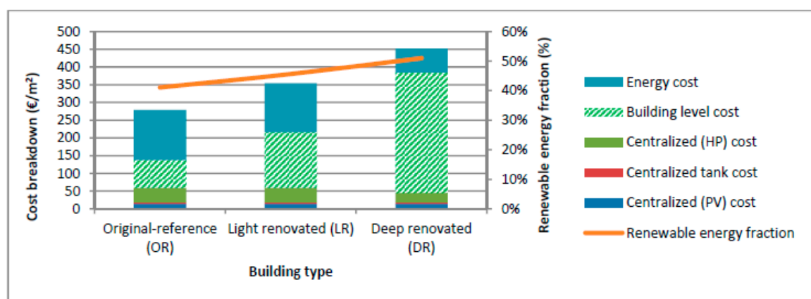
Figure 12. The breakdown of LCC of the old residential building community and the centralized PV and A2WHP-based energy system (Case 2, PV + A2WHP).
