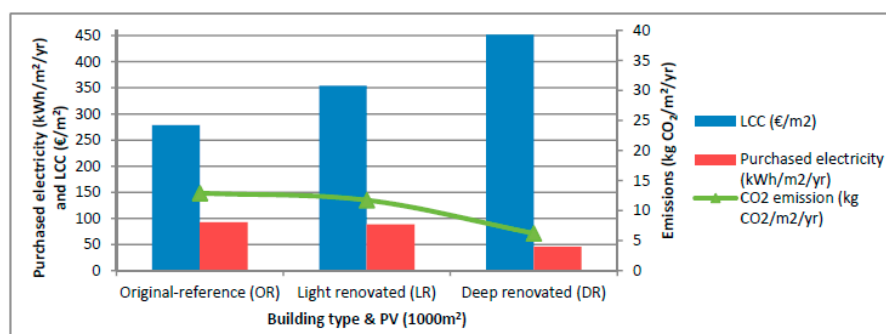
Figure 11. The annual purchased electricity, LCC, and CO 2 emissions from the centralized community-level PV and A2WHP-based energy system integrated with old residential buildings (Case 2, PV + A2WHP).
