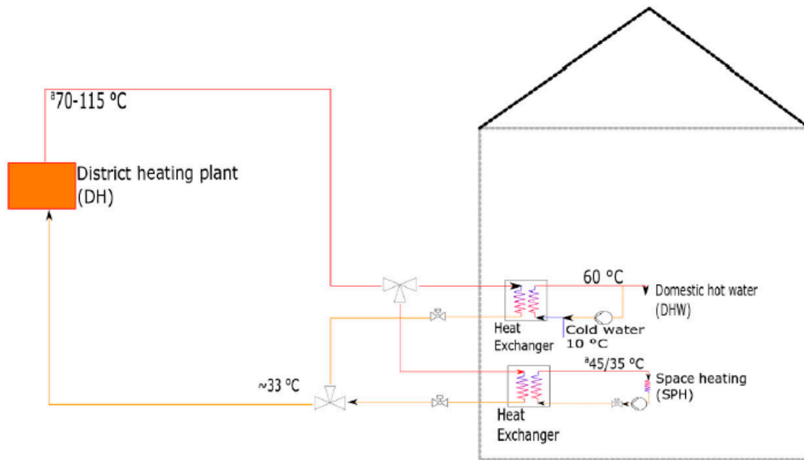
Figure 2. The schematic diagram of the reference old buildings integrated with city-level district heating (Case 0).
