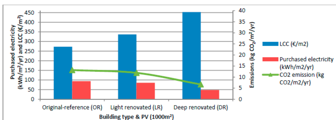
Figure 9. The annual purchased electricity, LCC, and CO 2 emissions from the centralized community-level PV and GSHP-based energy system integrated with old residential buildings (Case 1, PV + GSHP).
