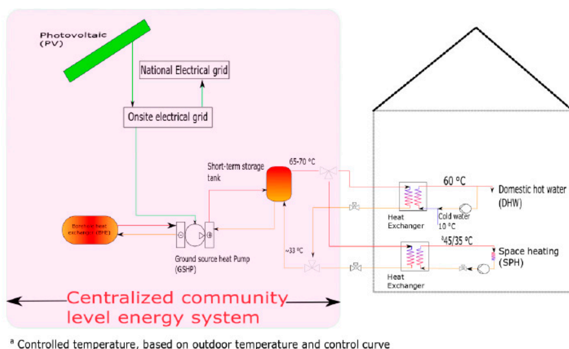
Figure 3. The schematic diagram of the centralized photovoltaic (PV) and ground source heat pump (GSHP)-based community-level district heating system integrated with old residential buildings in the district (Case 1, PV + GSHP).
