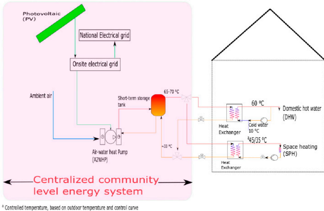
Figure 4. The schematic diagram of the centralized PV and A2WHP-based community-level district heating system integrated with old residential buildings in the district (Case 2, PV + A2WHP).
