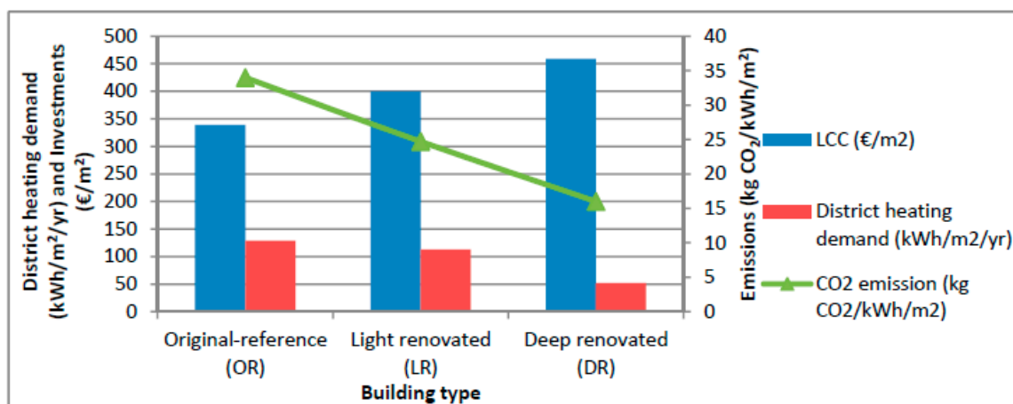
Figure 8. The annual heating demand of the buildings in the community, investment cost at the building level, and CO 2 emissions from the city-level district heating grid for the reference case (Case 0).
