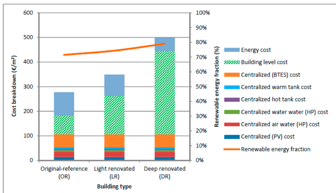
Figure 14. The breakdown of LCC of the old residential building community and centralized PV, HP and seasonal storage-based energy system (Case 3, PV + A2W + GSHP + STR).
