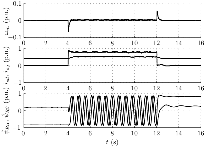
Fig. 9. Experimental results showing zero-speed operation when rated-load torque step is applied. Proposed gains were used. First subplot shows measured speed (solid) and estimated speed (dotted). Second subplot shows d and q components of stator current (solid) and their references (dashed) in estimated flux reference frame. Third subplot presents real and imaginary components of estimated rotor flux in stator reference frame.
