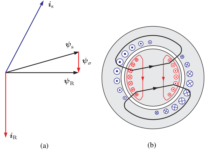
Fig. 3. (a) Space vector diagram and (b) magnetic flux paths: stator flux and rotor leakage flux.
