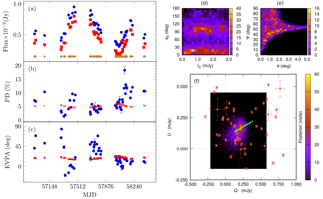
Fig. C.1. Results of polarisation analysis for VER J0521+211. Panel a: observed optical R -band flux (blue circles), variable component model (red squares), and model constant component (brown diamonds). Panel b: observed (blue circles) and modelled (red stars) optical polarisation degree. Panel c: observed (blue circle) and modelled (red triangles) electric vector polarisation angle. Panels d–f: posteriori distributions of the polarisation fitting. The colour scale gives the number of visits by the sampler in each cell. In addition, panel f shows the observations in the Q-U plane (orange) and evolution of the model (light green).
