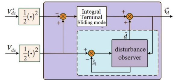
FIGURE 8. Illustration of voltage regulation loop with disturbance-observer- based ITSMC.
