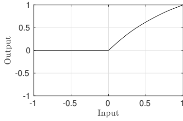
Figure 4: HWR-FEXP1 transfer function is a combination of a half-wave rectifier and an exponential function.
