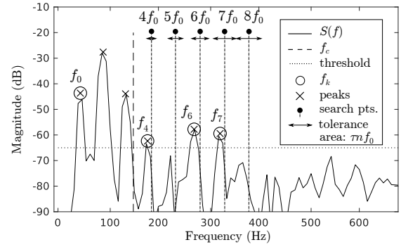
Figure 6: Example of harmonic detection when f_0 \in [\frac{1}{4}f_c, \frac{1}{3}f_c] .
