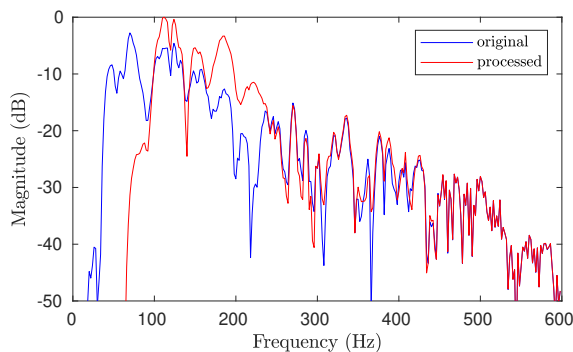
Figure 5: Effect of NLD processing on the spectrum of a kick drum sound, when the cutoff frequency is 120 Hz.
