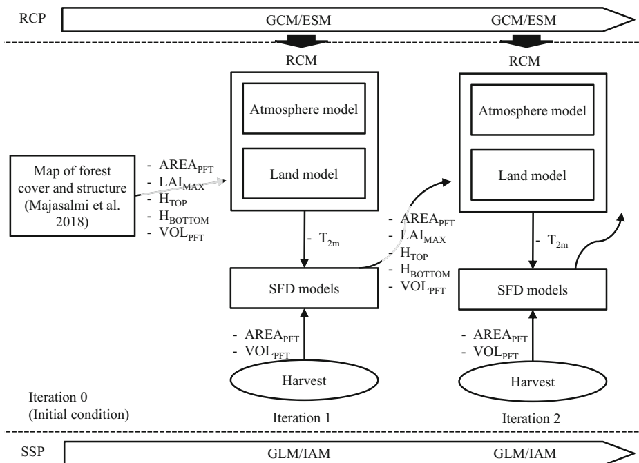
Fig. 1 Schematic illustrating the application F2S2's simple forest dynamic (SFD) models in asynchronously coupled regional climate modeling research. Abbreviations: AREA_{PFT} = area dominated by plant functional type (PFT) development class, LAI_{MAX} = Maximum growing season leaf area index, H_{TOP} = tree height, H_{BOTTOM} =canopy height, VOL_{PFT} = stem volume density, GCM= General Circulation Model, ESM= Earth System Model, RCM= Regional Climate Model, GLM= Global Land Model, IAM= Integrated Assessment Model, RCP= Representative Concentration Pathway, SSP= Shared Socio-economic Pathway
