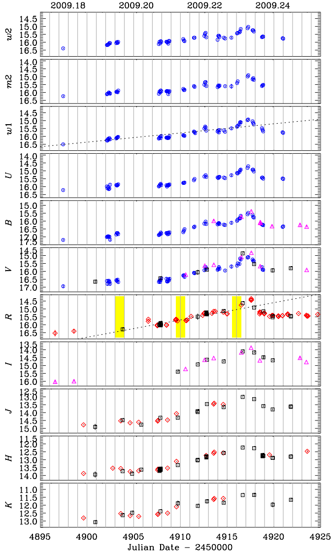
Fig. 3. Light curves collected in near-IR, optical and UV bands, between 5 March and 2 April 2009 (JD 2454895.5–2454924.5). Blue circles represent the UVOT data in v , b , u , uw1 , uwm2 , uw2 filters. Red diamonds represent GASP data in R , J , H , and K bands. Magenta triangles represent WEBT data in I , V , and B bands. REM data in V , R , I , J , H , and K bands are represented with black squares. Yellow regions in R -band light curve indicate the peaks of \gamma -ray activity observed by AGILE.
