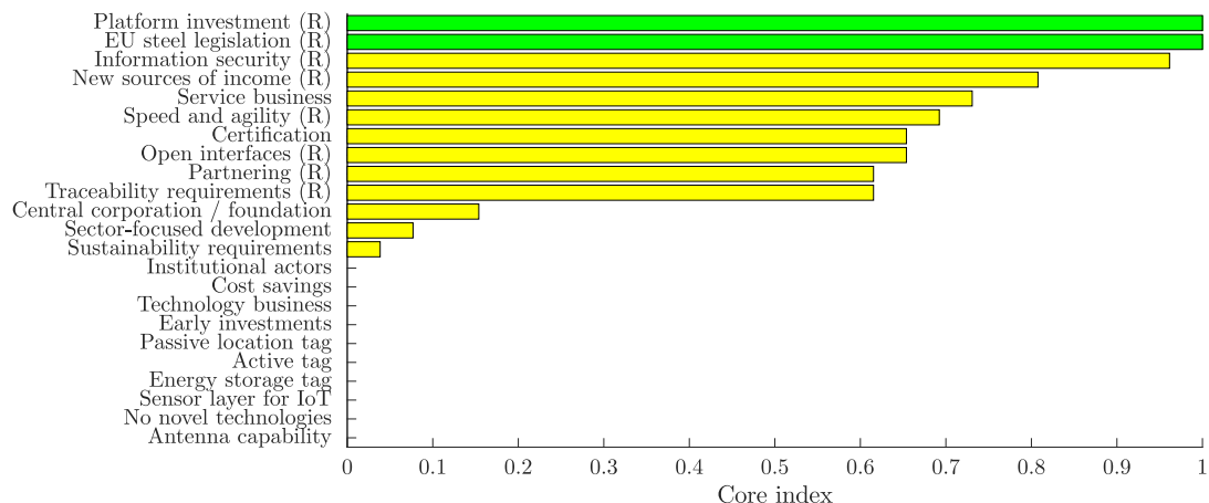
Fig. 12. Core indices corresponding to the 26 non-dominated portfolios, when the limit on the number of selected actions is b = 8 . Actions included in the portfolio recommended by both maximin and minimax regret decision rules are marked with (R).
