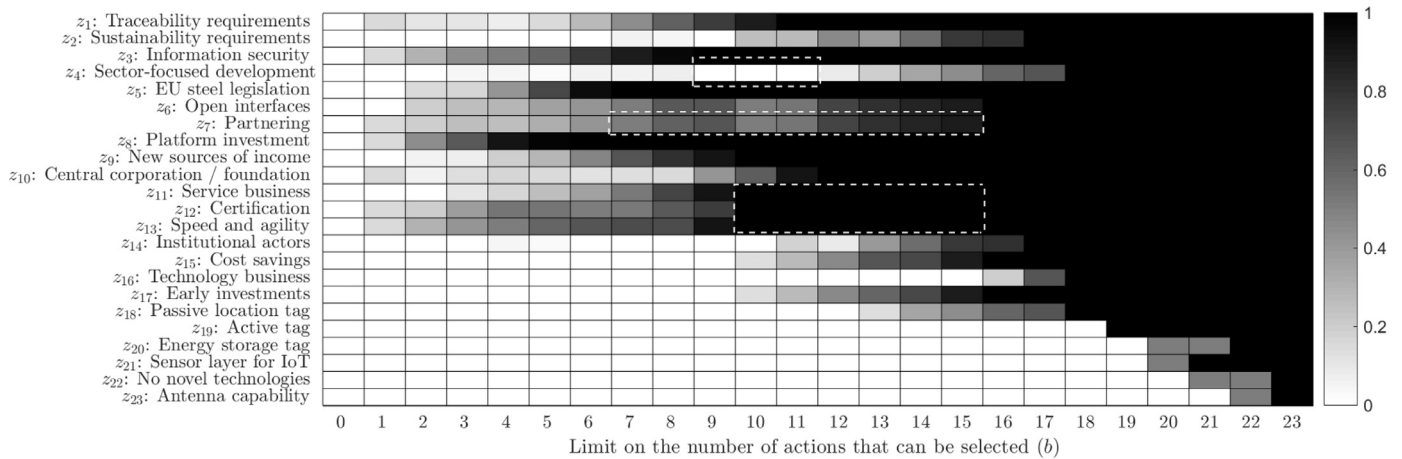
(a) Actions' core indices, when action-dependent probability information is taken into account.
