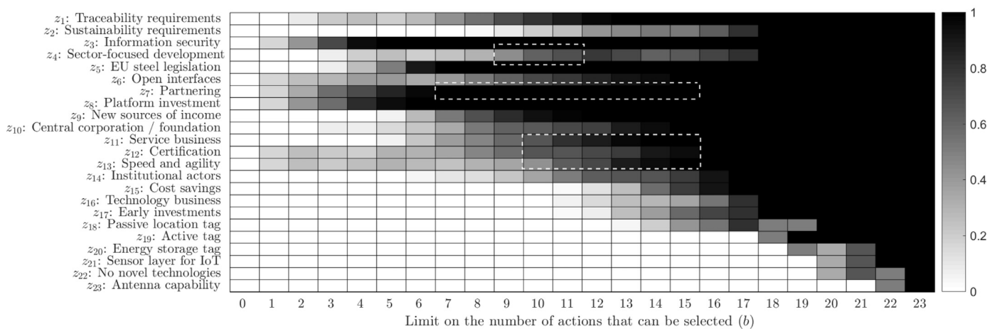
(b) Actions' core indices, when action-dependent probability information is neglected.
