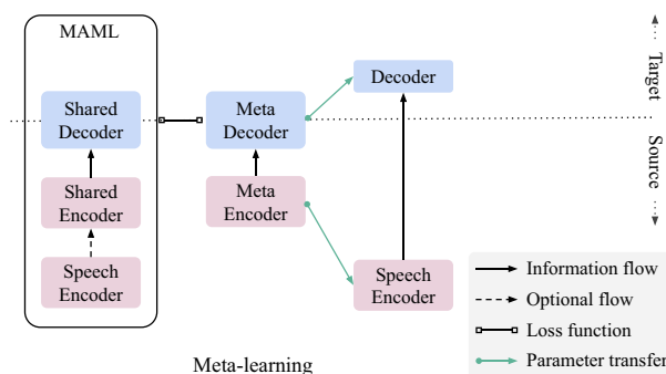
Fig. 9 Meta-learning expressed in the visual terms of the learning setups in Fig. 8. Meta-learning can be used to find a good initialization for standard training. The MAML algorithm explicitly learns to learn fast on the ASR and MT tasks
