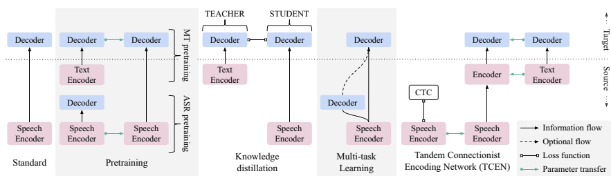
Fig. 8 Learning setups for end-to-end SLT: The standard framework uses untranscribed SLT data. Auxiliary data can be exploited in different ways such as by pretraining the encoder through ASR, pretraining the decoder through MT, knowledge distillation , or multi-task learning . The optional link in multi-task learning results in 2-step decoding. TCEN combines multiple types of pretraining
