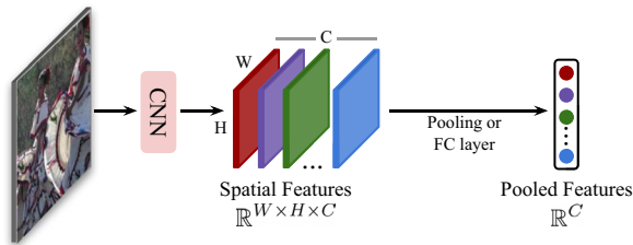
Fig. 5 An overview of two common types of visual featurers extracted from CNNs
