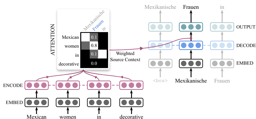
Fig. 4 A simplified view of encoder-decoder architecture with attention: an English sentence is first encoded into a latent space from which an attentive decoder sequentially generates the German sentence. The dashed recurrent connections are replaced by self-attention in fully-connected architectures such as transformers (Vaswani et al. 2017)
