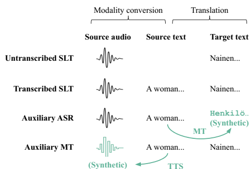
Fig. 7 Four types of data that can be used to train SLT systems. Untranscribed SLT is the minimal type of data for end-to-end systems. Adding source text transcripts completes the triple. The source text is an intermediate representation which divides the SLT mapping into a modality conversion and a translation. Two types of auxiliary data, ASR and MT data, form adjacent pairs in the triple, leaving one of the ends empty. The auxiliary data can be used as is for pretraining or multi-task learning, or it can be completed into synthetic triples using external TTS or MT systems
