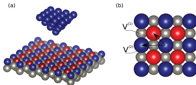
Fig. 2 (a) Illustration of the simulated system when the cluster at the tip is modeled as a four layer pyramid containing 30 Fe atoms. The atoms in the antiferromagnetic Fe overlayer are shown in blue/red to indicate parallel/antiparallel ordering of the magnetic moment with respect to the cluster at the tip. The underlying W atoms are shown in grey. The atoms at the boundary of the simulation cell are shown twice for clarity (but are equivalent because of periodic boundary conditions). (b) Since the distance between the atoms in the Fe overlayer is large, they interact through the conductivity band of the W substrate. The arrows indicate the interaction between first- and second-neighbor Fe atoms. There are twice as many Fe–W–Fe paths between first neighbors than second neighbors, so the hopping parameters in the NCAA models are chosen such that V^{(2)} = V^{(1)}/\sqrt{2} .
