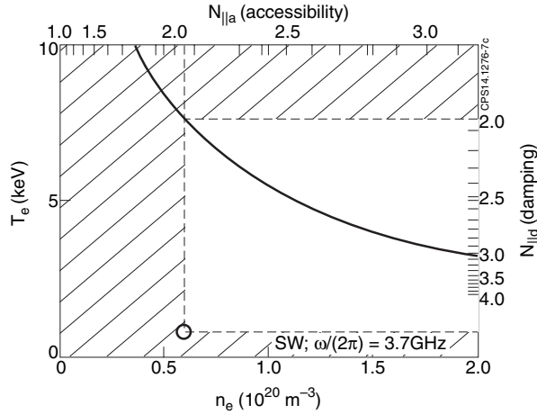
Figure 7. LHCD accessibility diagram at 3.7 GHz.
