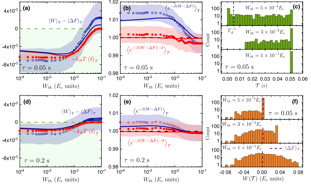
FIG. 3. Dissipated work \langle W \rangle_{\mathcal{T}} - \langle \Delta F \rangle_{\mathcal{T}} (blue) and stochastic indistinguishability at stopping times (red) -k_B T \langle \delta(\mathcal{T}) \rangle (dots: experimental data; solid lines: simulation) in charging energy E_c = 109 \mu\text{eV} units averaged over many realizations for protocol durations \tau = 0.05 s (a) and \tau = 0.2 s (d) as a function of work threshold values. (b),(e) Test of the generalized work fluctuation relation and of Eq. (3) (dots: experimental data; solid lines: simulation) for \tau = 0.05 s (b) and \tau = 0.2 s (e). (c),(f) Histograms of stopping times \mathcal{T} (c) and corresponding work values W(\mathcal{T}) (f) for a ramp time \tau = 0.05 s for work thresholds W_{th} = 5 \times 10^{-4}, 3 \times 10^{-2} and 10^{-1} E_c . The total uncertainty is shown by shadowed areas; it is the combination of the statistical uncertainty and error on temperature (about 10%).
