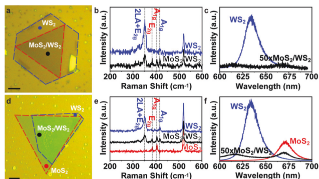
Fig. 2 Optical characterization of the \text{MoS}_2/\text{WS}_2 heterostructure. (a) Optical microscopy images of the heterostructures (scale bar, 10\ \mu\text{m} ). (b) Raman and (c) PL spectra at the marked dots with the same colours, respectively (black PL spectrum with 50 times magnification). (d) Optical microscopy images of a partial stacking heterostructure (scale bar, 25\ \mu\text{m} ). (e) Raman and (f) PL spectra at the marked dots with the same colours, respectively (black PL spectrum with 50 times magnification).
