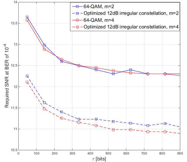
Fig. 2: The required SNR values of SNR-adaptive optimized 64-ary signalling model and SNR-independent 64-QAM model where rate-1/2 ([5, 7]_8) convolutional encoder is used for all cases.
