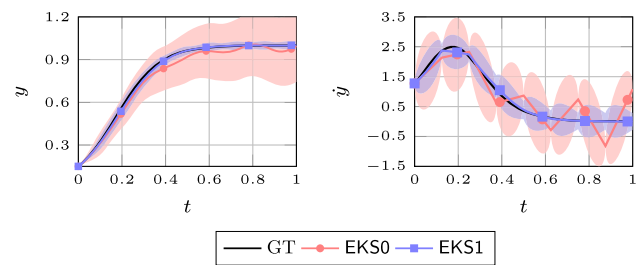
Fig. 3 Reconstruction of the logistic map (left) and its derivative (right) with two standard deviation credible bands for EKS0 (red) and EKS1 (blue). (Color figure online)
