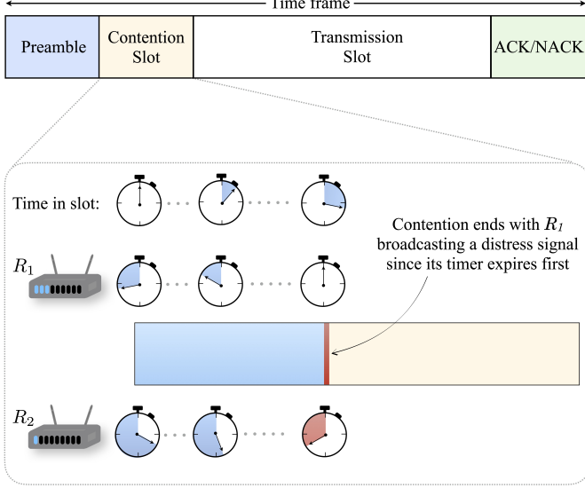
Fig. 2. A simple example of how the timer-based approach works for a network of two relays. The relay with more packets in its buffer has its timer expire first during the contention period.
