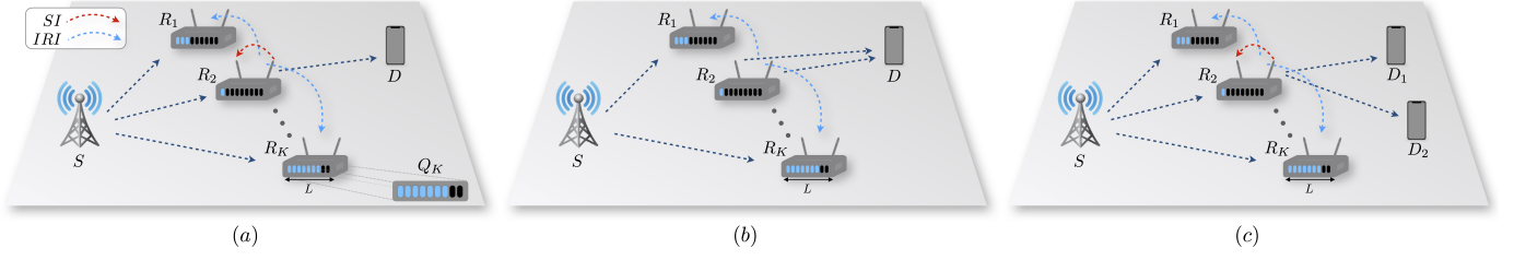
Fig. 1. The topology of a buffer-aided full-duplex relay network: (a) Full-duplex relaying, (b) successive relaying and (c) full-duplex NOMA transmission.
