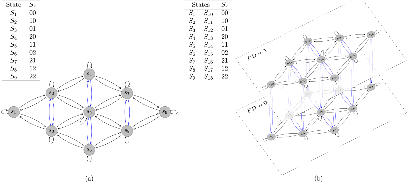
Fig. 3. Markov chain for different scenarios: (a) When no FD transmissions are available (e.g., because of HD relays), single transmissions within a slot are represented by black lines, whereas SuR with blue lines. (b) Full-duplex relaying requires one more level to depict the transmission, due to the fact that the state of the buffers remains unchanged.
