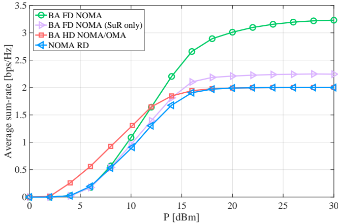
Fig. 4. Average sum-rate for K = 3 , L = 4 and various algorithms.
