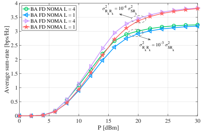
Fig. 5. Average sum-rate for K = 3 , varying L and SI channel conditions.
