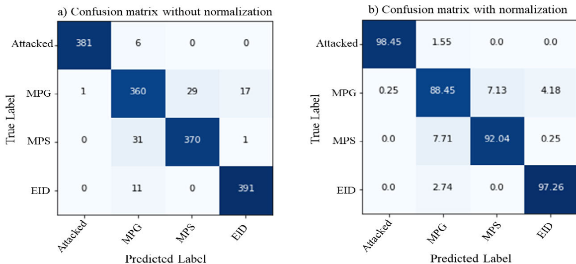
FIGURE 7. Classification result from proposed DT; (a) Confusion matrix without normalization, and (b) Confusion matrix with normalization.
