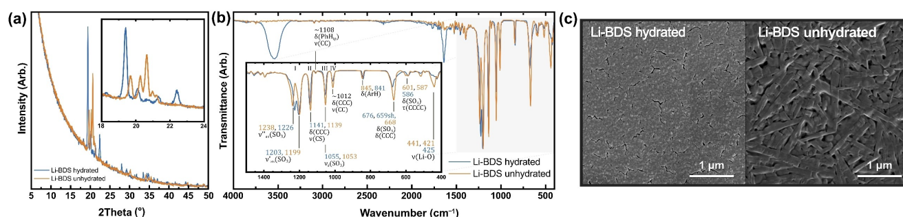
Figure 4. (a) GIXRD patterns of hydrated and unhydrated Li-BDS films (800 cycles at 200 °C). Inset shows a magnification between 18° and 24° to highlight the differences in the pattern. (b) Representative FTIR spectra of hydrated (800 cycles at 200 °C) and unhydrated Li-BDS spectra with inset highlighting the minor differences in the 1500 to 400 cm −1 range. Peak interpretation of the FTIR spectra is also included in the inset with blue (Li-BDS hydrated) and orange (Li-BDS unhydrated) color coding listing the wavenumbers. The roman numerals I–IV highlight the most typical peaks of metal-BDS compounds. A detailed discussion of the FTIR spectrum can be found in the Supporting Information. The symbols are \nu for stretch, \delta for bending, and \tau for torsion. (c) SEM images of the Li-BDS films. Hydrated film is imaged directly after deposition while the unhydrated sample was stored in desiccator for 24 h prior imaging.
