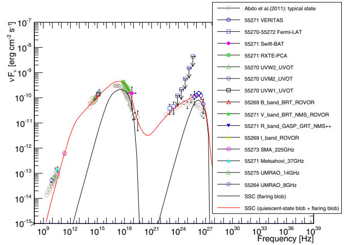
(f) MJD 55 271.
