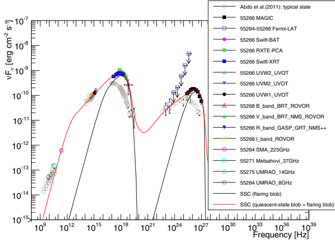
(a) MJD 55 266.
