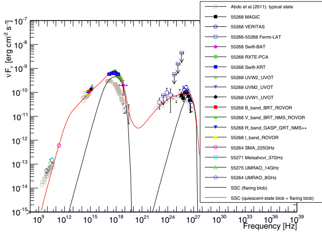
(c) MJD 55 268.
