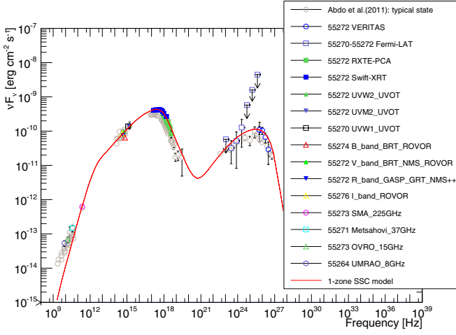
(a) MJD 55 272.
