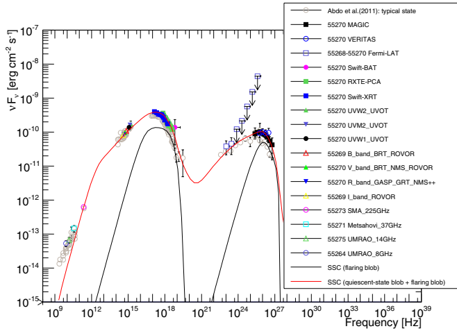
(e) MJD 55 270.
