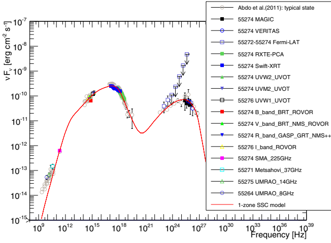
(c) MJD 55 274.
