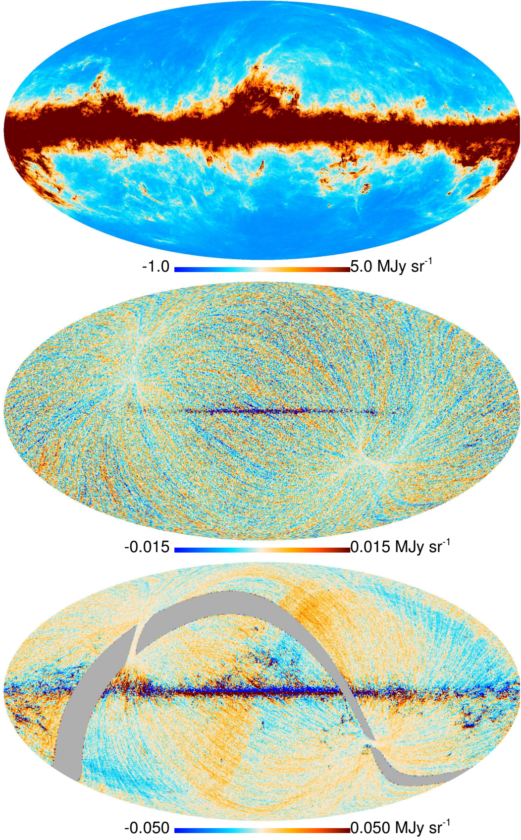
Fig. 19. HFI maps at 545 GHz. The top panel gives the intensity in \text{MJy sr}^{-1} . The middle panel shows the difference between maps made from the first and the second halves of each stable pointing period (i.e., half-ring maps). The bottom panel shows the difference between Survey 1 and Survey 2.
