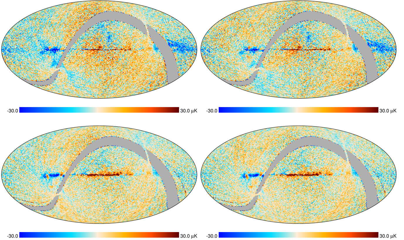
Fig. A.1. Top: data difference maps for the 143-GHz bolometer. Bottom: differences from a simulation including the effect of ADC non-linearity and 4 K lines. Left column: Survey 1–Survey 2 differences for maps made without destriping. Right column: Survey 1–Survey 2 differences after the destriping used to create the delivered data. The match is sufficiently good that one can use such simulations to estimate the combined effect of the non-linearity of the ADC on the delivered data.
