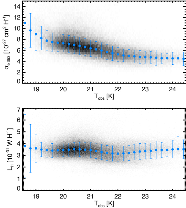
Fig. 19. Variation of \sigma_{e353} (upper) and L_{\text{H}} (lower) as a function of T_{\text{obs}} in the diffuse ISM. Data used were smoothed to 30' , the angular resolution of the HI data. Only pixels where 1 \times 10^{20} < N_{\text{HI}} < 2.5 \times 10^{20} \text{ cm}^{-2} were selected. The greyscale shows the point density in the two-dimensional histogram while the blue points indicate the average and standard deviation of L_{\text{H}} and \sigma_{e353} in bins of T_{\text{obs}} .
