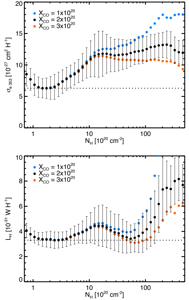
Fig. 20. \sigma_{e353} (upper) and L_{\text{H}} (lower) vs. N_{\text{H}} computed at 30' resolution from Eq. (13) with three values of X_{\text{CO}} : [1, 2, 3] \times 10^{20} \text{ H}_2 \text{ cm}^{-2} \text{ K}^{-1} \text{ km}^{-1} \text{ s} . The mean values of \sigma_{e353} and L_{\text{H}} were computed in bins of N_{\text{H}} equally spaced in log; the error bar is the standard deviation, shown only for X_{\text{CO}} = 2 \times 10^{20} \text{ H}_2 \text{ cm}^{-2} \text{ K}^{-1} \text{ km}^{-1} \text{ s} . The horizontal dotted line indicates the average values found in the low N_{\text{HI}} mask.
