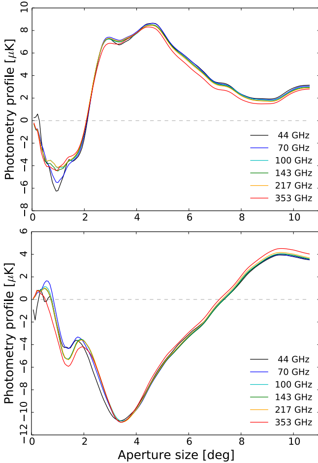
Fig. 8. Coherence of the signal across the SEVEM frequency channels. The aperture photometry profiles measured in the stacked patches centred on superclusters ( top ) and supervoids ( bottom ) are virtually identical for all frequencies, as it is expected for the ISW signal.
