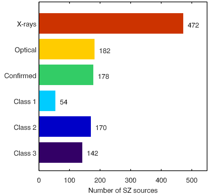
Fig. 18. Distribution of the Planck clusters and candidates in the different categories defined in the external validation process. The validation follows the order of association with MCXC clusters, then Abell and Zwicky clusters, then SDSS clusters, then SZ clusters, and finally clusters from NED/SIMBAD.
