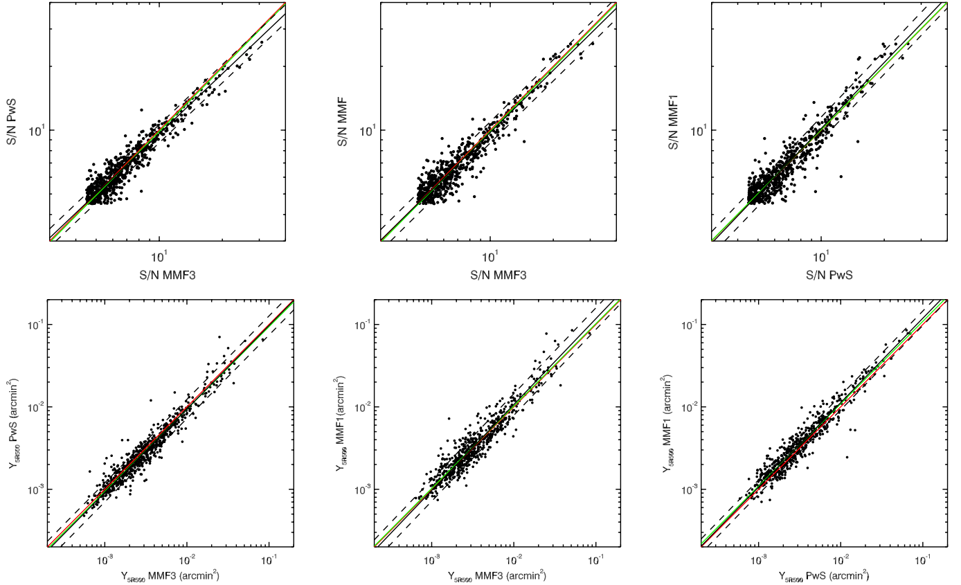
Fig. 6. Comparison of S/N ( top panels ) and maximum likelihood Compton-parameter values ( bottom panels ) from the three detection algorithms, MMF3 and PwS, down to S/N = 4.5 after removing obvious false detections (see Sect. 2.3). In each panel, the red line denotes the equality line. The black line is the best fit to the data, and the dashed lines correspond to the \pm 1\sigma dispersion about the fit relation. For clarity, error bars are omitted on Y_{5R500} values in the plot, but are taken into account in the fit. The green line of slope fixed to unity corresponds to the mean offset between the two quantities. Numerical results for the fits are given in Table 1.
