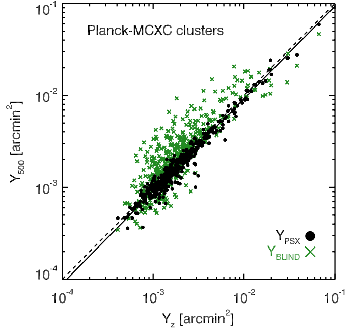
Fig. 26. Comparison of the different Y estimates for the Planck clusters identified with MCXC clusters. In green are the blind measured Y values and in black are the refined Y_{500,\text{PSX}} measured fixing the size and positions to the X-ray values. Both are plotted as a function of the new proxy Y_z .
