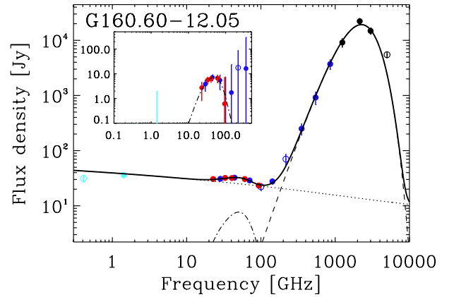
Fig. 17. SED for G160.60–12.05 (California nebula). The curves and symbols are as in Fig. 8. AME is detected at a level of \sigma_{AME} = 5.0 , and the best-fitting spinning dust peak is shifted to \nu_{sp} = (50 \pm 17) GHz.
