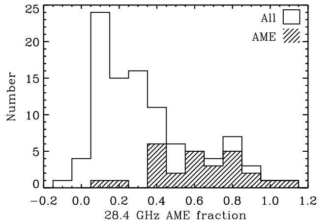
Fig. 11. Histogram of the AME fraction, S_{28}^{28_{\text{resid}}}/S_{28} , at 28.4 GHz. The total sample is shown as the unfilled histogram, while significant ( \sigma_{\text{AME}} > 5 ) AME sources are in the hatched region.
