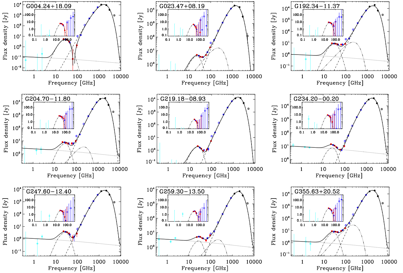
Fig. 8. SEDs for the sources with very significant AME and f_{\text{max}}^{\text{UCH II}} < 0.25 . Data points are shown as circles with errors and are colour-coded for radio data (light blue), WMAP (red), Planck (blue), and DIRBE/IRAS (black). The best-fitting model of free-free (dotted line), thermal dust (short-dashed line), CMB (triple-dot dashed line), and spinning dust (dot-dashed line) is shown. Data included in the fit are shown as filled circles, while the other data are unfilled. The residual spectrum, after subtraction of free-free, synchrotron, CMB, and thermal dust components, is shown in the insert . The best-fitting spinning dust model is also shown.
