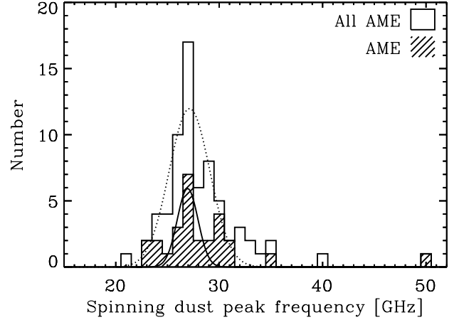
Fig. 16. Histogram of spinning dust peak frequencies, \nu_{sp} . The unfilled histogram is for both AME and semi-significant AME regions, while the hatched region is for the AME sources only. The best-fitting Gaussians for these two histograms are overplotted. The source at \nu_{sp} = 50 GHz is G160.60–12.05 (California nebula).
