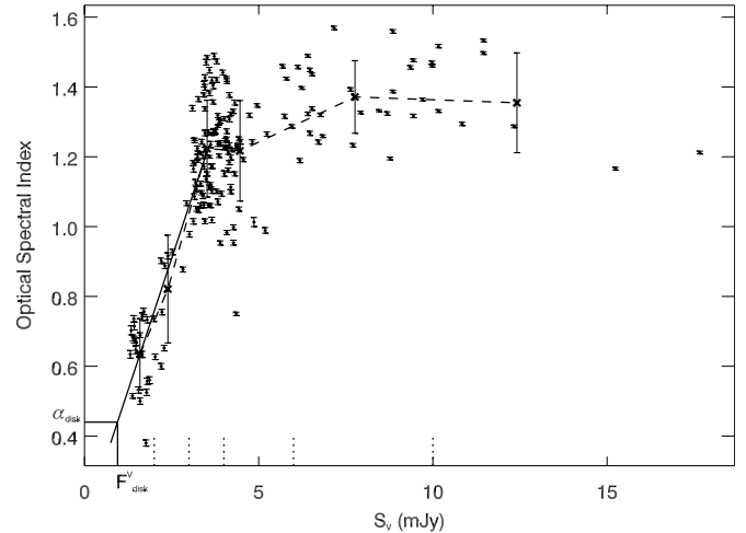
Figure 19. Spectral index vs. brightness of the optical continuum in V band in the observer's frame; crosses show average values of \alpha_{\text{cont}} within different intervals of flux, S_V (Table 6), connected by the dashed line; dotted vertical segments show intervals of the averaging; the solid line is a linear fit of the dependence for S_V < 4.0 mJy.
