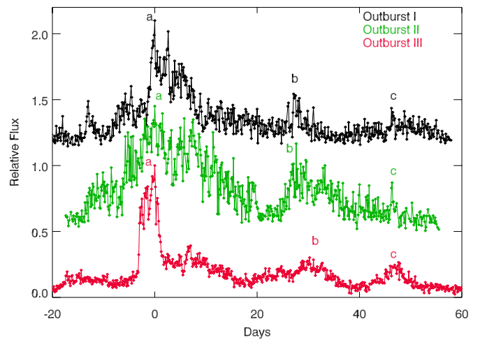
Figure 3. Gamma-ray light curves during outbursts I (black), II (green), and III (red) relative to T_\gamma^{\max} of each outburst and normalized to corresponding S_\gamma^{\max} ; light curves I and II are shifted by 1.1 and 0.45, respectively, for clarity. The three main flares during each outburst are designated as a , b , and c (see Table 1).
