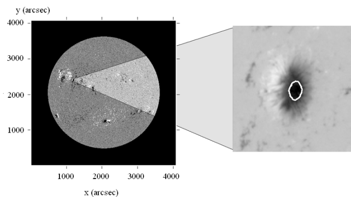
Fig. 2. Left panel: SDO/HMI magnetogram of a full solar disk. Right panel: contour of the sunspot umbra at the level of 1000 G, obtained from the active region NOAA 11251.
