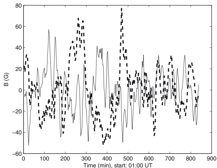
Fig. 9. SDO/HMI magnetic field time-series obtained from the magnetograms of the two distant sunspots NOAA 11242 (N17, W29) and NOAA 11243 (N16, E38). Date of observations: 2011/06/30.
