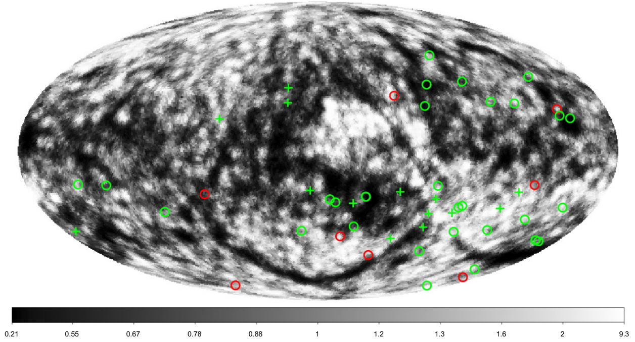
Fig. B.1. XMM-Newton validation results overplotted on density map of the RASS-Bright Source Catalogue (BSC). The source density map has been normalised by the median of the pixel density distribution. Confirmed candidates are plotted in green and false candidates are plotted in red. Pluses (+): good association with a BSC source. Circles (○): no association with a BSC source.
