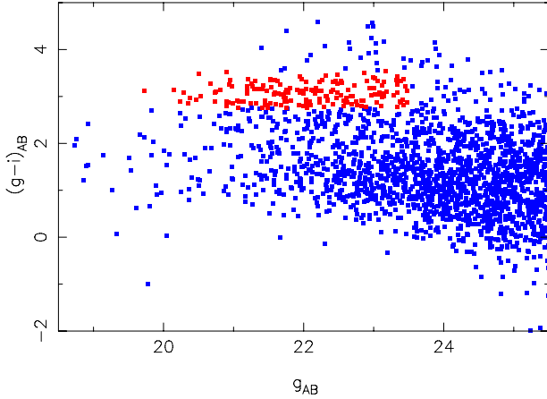
Fig. A.2. A g-i vs. g colour-magnitude diagram of non-stellar objects in the field of PLCK G147.3–16.6, observed with NOT/MOSCA. Galaxies plotted as red squares, in the region defined by g-i = 3.15 \pm 0.40 and g < 23.5 , form the red sequence constituted by early-type galaxies in the cluster.
