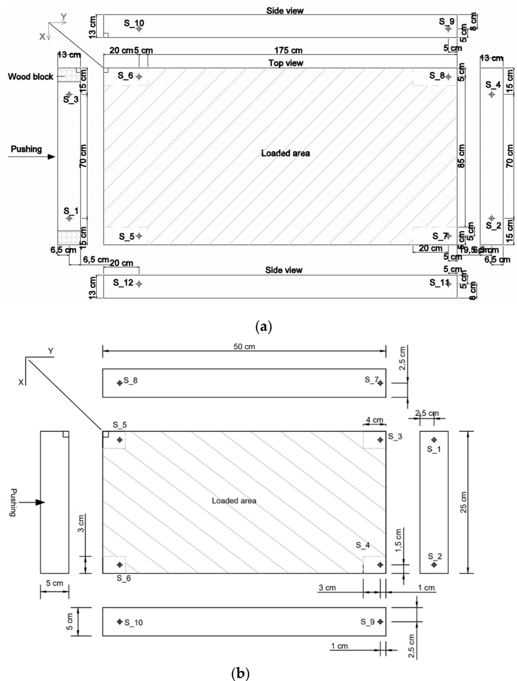
Figure 5. Layout of the locations of the displacement sensors: (a) large, and (b) medium. The positions of the linear variable differential transformers (LVDTs) are shown by the symbol S.
