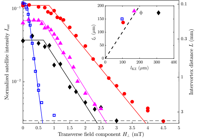
FIG. 2. Suppression of the HQV density created by the KZM as a function of the applied bias. Filled red circles, magenta triangles, and black diamonds correspond to quench rates of \tau_Q \approx 3.8 \times 10^2 \text{ s} , \tau_Q \approx 1.4 \times 10^3 \text{ s} , and \tau_Q \approx 7.7 \times 10^3 \text{ s} , respectively, while applying a constant H = 11 \text{ mT} magnetic field. The field is rotated to achieve different bias fields H_{\perp} = H \sin \mu . Open blue squares ( \tau_Q \approx 6.0 \times 10^2 \text{ s} ) correspond to measurements with zero axial field component, H_{\perp} = H . Vortex density is constant for H_{\perp} < H_{\perp t} and suppressed for higher bias fields. The suppression starts when the characteristic length scale of the bias field \xi_{\text{bias}}(H_{\perp}) becomes smaller than the relevant Kibble-Zurek length. Solid lines correspond to theoretical model (see text for details). The dashed line shows where the intervortex distance becomes comparable with the container size. The inset shows the extracted threshold bias length \xi_t as a function of l_{\text{KZ}} with the same symbols. The dashed line is \xi_t = l_{\text{KZ}} . The patterned gray diamond is the same measurement as the black diamond, but with l_{\text{KZ}} on the horizontal axis replaced with an estimation of the transition front thickness l_F [15]. For other measurements, l_F lies beyond the right border of the plot.
