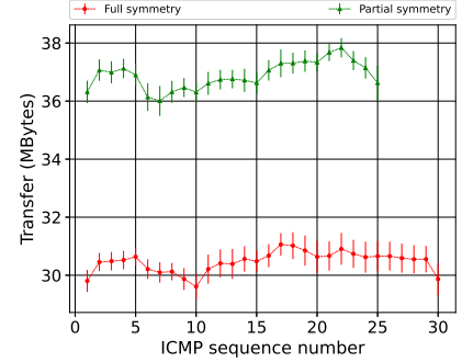
(b) Transfer variation in time for full and partial symmetry scenarios.
