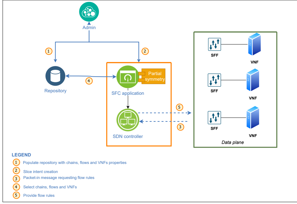
Fig. 4: System architecture for implementing the partial symmetry SFC.
