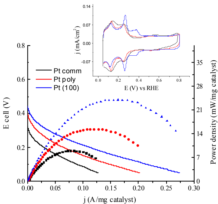
Figure 2 – Polarization and power density curves obtained for Pt comm, Pt poly and Pt (100) as anode catalysts obtained from the fuel cell measurements at 70 °C, with 1 M ethanol as fuel and 200 ml/min O 2 as oxidant. Inset: Cyclic voltammograms for Pt comm, Pt poly and Pt (100) in 0.5 M H 2 SO 4 , 50mV/s.
