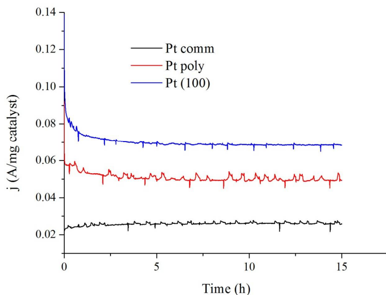
Figure 3 – Chronoamperometry curves for Pt comm, Pt poly and Pt (100) as anode catalysts obtained at 0.2 V, at 70 °C with 1 M ethanol as fuel and 200 ml/min O 2 as oxidant.
