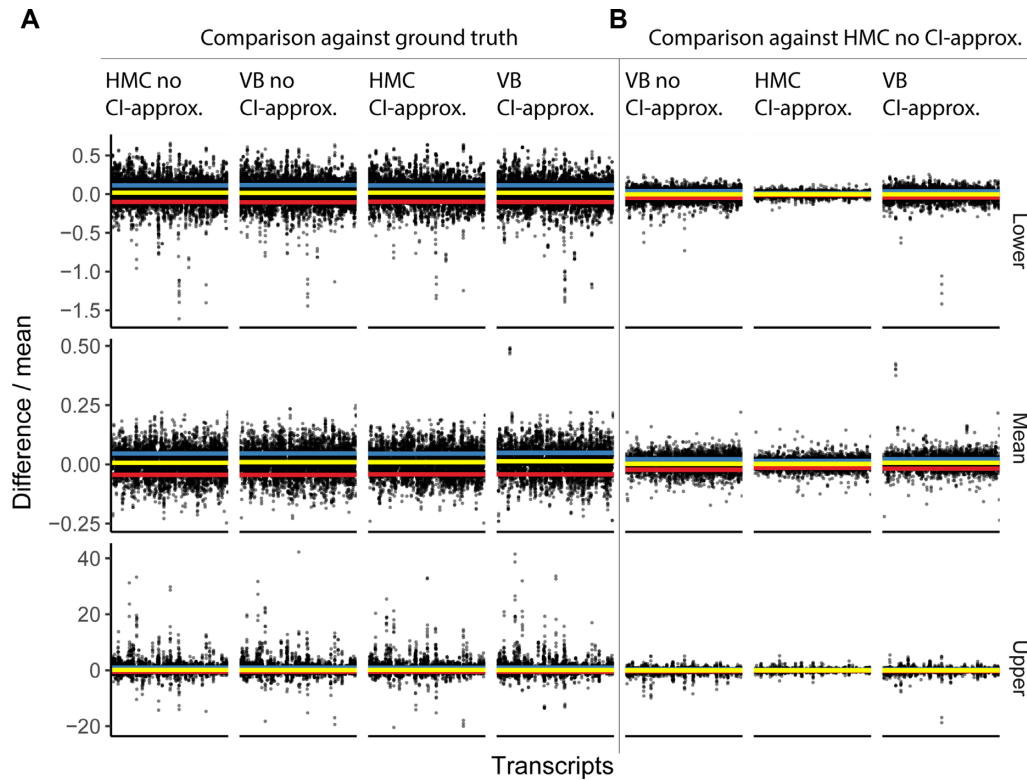
Figure 5. Evidence that the use of both variational Bayes and credible interval (CI) approximation does not significantly affect the inference compared with the Hamiltonian Monte Carlo sampler. These tests were performed on simulated data from the joint posterior distribution fitted on real data (26) (see ‘Materials and Methods’ section). Each data point represents the inference for one gene. The y axis represents the scaled (by mean) difference of each method combination (specified in the header of the vertical facet strips) and the ground truth (specified in the panel headers). The three horizontal facet strips (lower, mean, and upper) include the inferred mean, and lower and upper quantiles (95% credible interval) of the theoretical data distributions. The yellow horizontal line corresponds to the median error, the blue and red lines correspond to the upper and lower standard deviation. (A) Comparison of the ground truth (simulated data) with (from left to right) Hamiltonian Monte Carlo sampling, variational Bayes, Hamiltonian Monte Carlo with credible interval approximation, and variational Bayes with credible interval approximation. (B) Comparison of the Hamiltonian Monte Carlo sampling (without any approximation) with variational Bayes (with and without credible interval approximation) and Hamiltonian Monte Carlo sampling with credible interval approximation.
