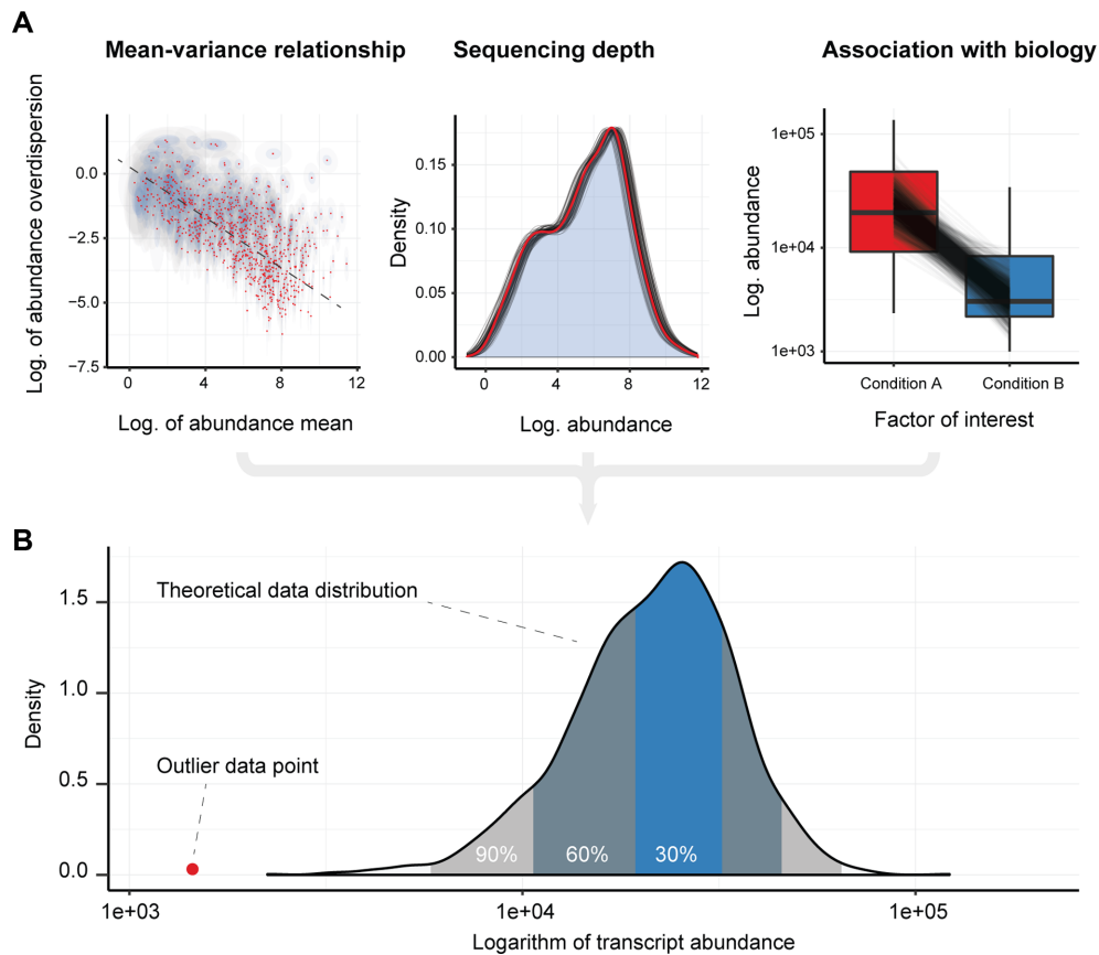
Figure 1. Graphical example of the estimation of the theoretical data distribution. The theoretical data distribution is estimated for each biological-replicate/transcript pair from the joint posterior distributions. (A) Left: the uncertainty of transcript-wise abundance baseline, where log-overdispersions are modelled in association with their log-mean. The point estimates are coloured in red, while the ellipses represent the 2D credible intervals 40% (blue) and 95% (grey); Middle: the density histogram of the posterior expected values for all genes for one biological replicate, adjusted by the exposure parameter (95% credible interval). The overlapping densities represent the uncertainty of the sequencing depth for one biological-replicate, modelled by the exposure parameter. The red curve corresponds with the adjustment for the mean of the posterior probability of the inferred exposure rate; Right: the uncertainty of the expected abundance values (95% credible interval) of a single transcript across two experimental conditions. The boxplots visualize the observed data distribution, while the black lines visualize the posterior densities of expected abundance according to the linear model. (B) An illustrative example of the theoretical transcript abundance distribution that is estimated for a biological replicate/transcript pair. Shaded regions correspond to central credible intervals of the distribution.
