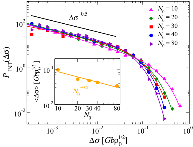
FIG. 4. Main figure shows the strain-integrated stress increment distributions P_{\text{INT}}(\Delta\sigma) for different N_0 , revealing a cutoff decreasing with the system size. The inset shows that the average stress jump magnitude \langle\Delta\sigma\rangle decreases as N_0^{-0.5} .
