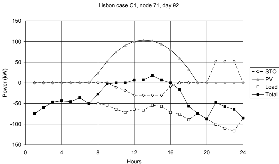
Figure 4.1: Typical day with storage charge-discharge cycle in Lisbon case C1.
