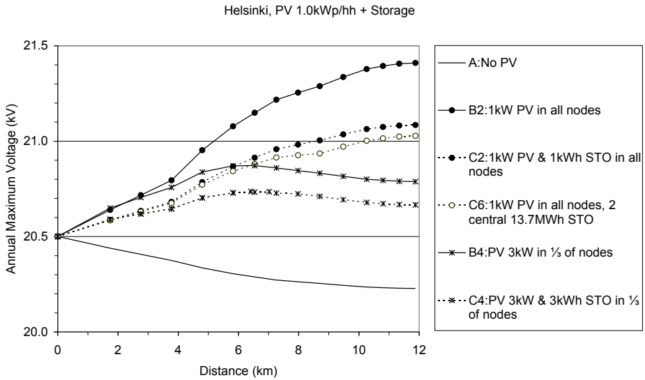
Figure 4.3: Annual maximum voltage profiles in Helsinki for cases A, B2, B4, C2, C4, and C6. The installed PV capacity totals 1.0 \text{ kW}_p / \text{hh} , and the corresponding storage capacity 1.0 \text{ kWh} / \text{hh} .
