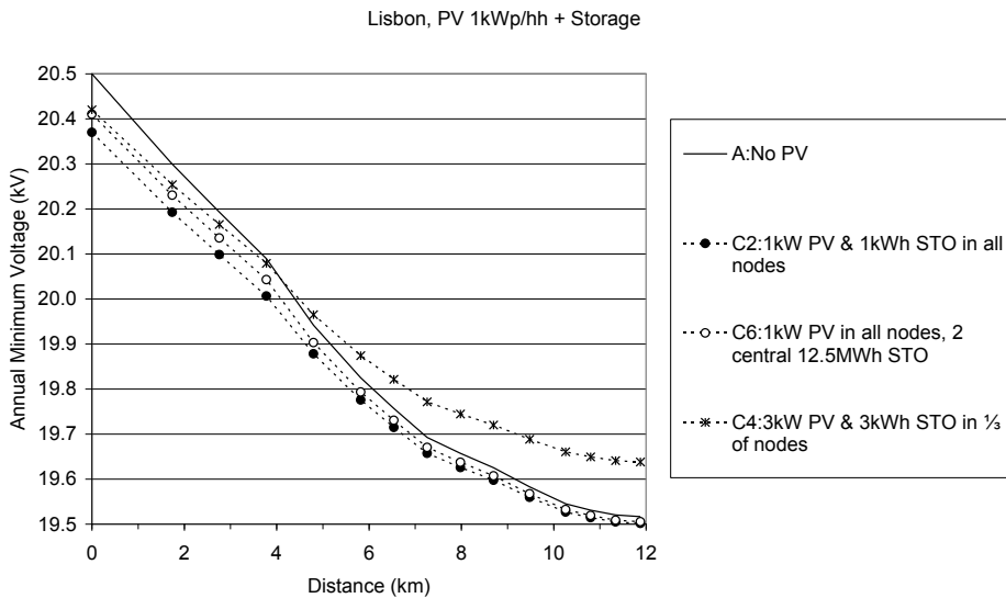
Figure 4.6: Annual minimum voltage profiles in Lisbon for cases A, C2, C4, and C6. The installed PV capacity totals 1.0 \text{ kW}_p / \text{hh} , and the corresponding storage capacity 1.0 \text{ kWh} / \text{hh} .
