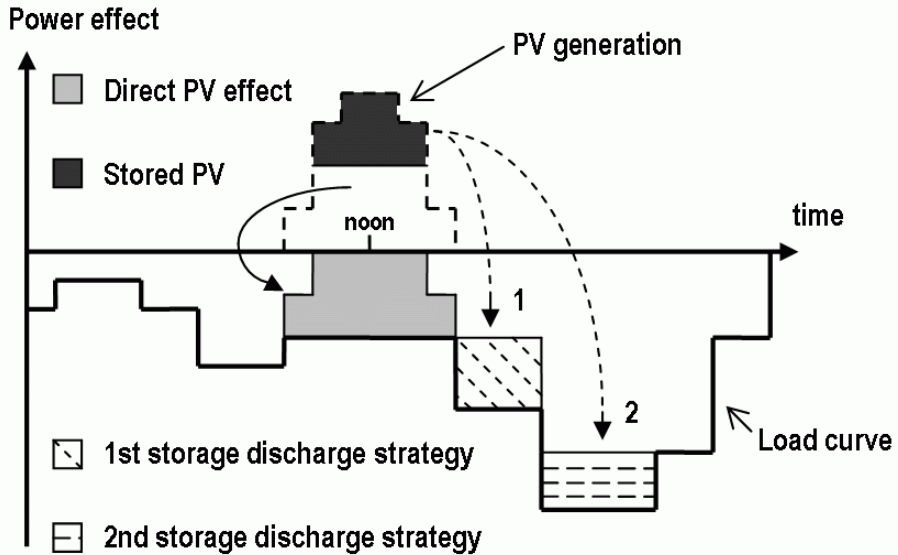
Figure 2.1: Schematic presentation of the two storage control strategies applied. The 1 st discharge strategy refers to non-optimized discharge, where no evening peak reduction is gained. The 2 nd strategy distributes the stored electricity evenly over the evening peak hours, reducing the evening peak correspondingly.
