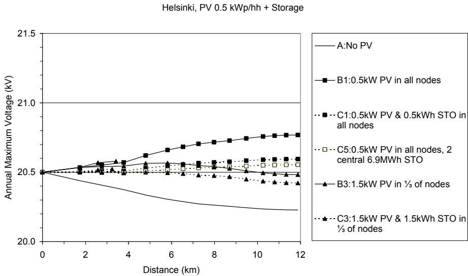
Figure 4.2: Annual maximum voltage profiles in Helsinki for cases A, B1, B3, C1, C3, and C5. The installed PV capacity totals 0.5 kW p / hh, and the corresponding storage capacity 0.5 kWh / hh.
