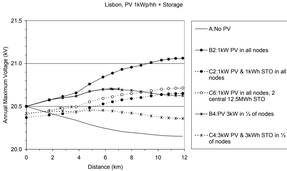
Figure 4.5: Annual maximum voltage profiles in Lisbon for cases A, B2, B4, C2, C4, and C6. The installed PV capacity totals 1.0 \text{ kW}_p / \text{hh} , and the corresponding storage capacity 1.0 \text{ kWh} / \text{hh} .
