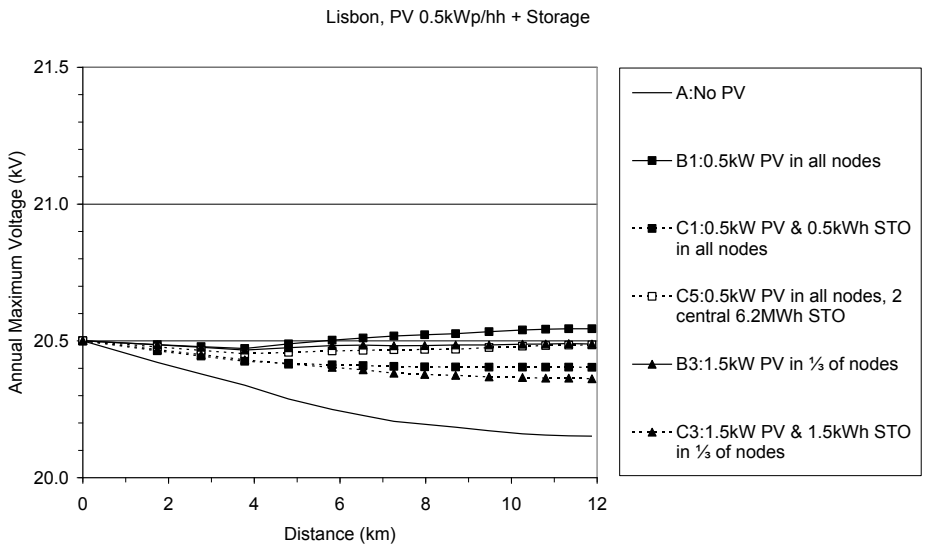
Figure 4.4: Annual maximum voltage profiles in Lisbon for cases A, B1, B3, C1, C3, and C5. The installed PV capacity totals 0.5 \text{ kW}_p / \text{hh} , and the corresponding storage capacity 0.5 \text{ kWh} / \text{hh} .
