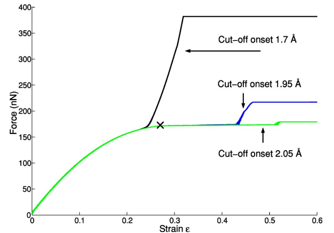
FIG. 1. Force-strain curves for an ideal (5,5)-nanotube at 10 K temperature with three different cut-off radii. The onset of the cut-off function can be perceived as an artificial peak. The flat regime depicts a sudden bond elongation to a length corresponding to the cut-off. Thus the beginning of this plateau, "X," corresponds to the largest value of force outside the cut-off peak and will be interpreted as bond rupture.
