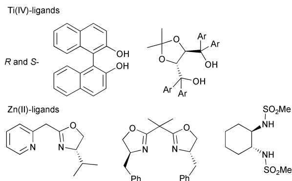
Fig. 1 Chiral ligands examined in the alkylation reaction shown in Scheme 2.
