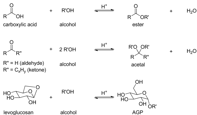
Scheme 1. Main Reactions between Fast Pyrolysis Bio-Oil and Alcohols: Esterification of Acids and Acetalization of Aldehydes, Ketones, and Sugars a
