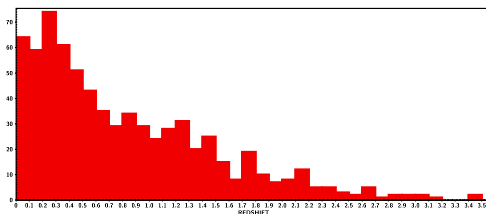
Figure 2. Redshift distribution of the checked sources.
