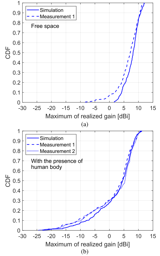
Fig. 12. Statistics of spherical coverage (a) in free space and (b) with the hexagonal body phantom (measurements) and the full numerical human model (simulations).
