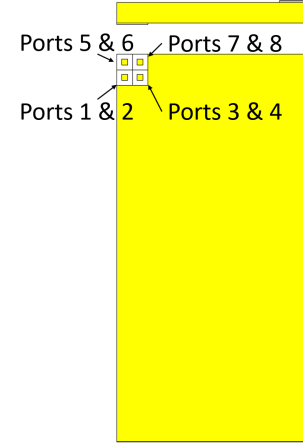
Fig. 5. Colocated array configurations, seen from front and top sides of the mobile phone chassis with one module on front- and one on back-side. Used in simulations (two discrete ports per element adding up to 16 ports in total).
