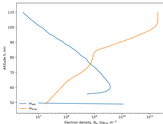
Figure 10. Fit of an electron density profile (SVD method). The discontinuity corresponds to the minimum altitude of the input collision frequency profile.
