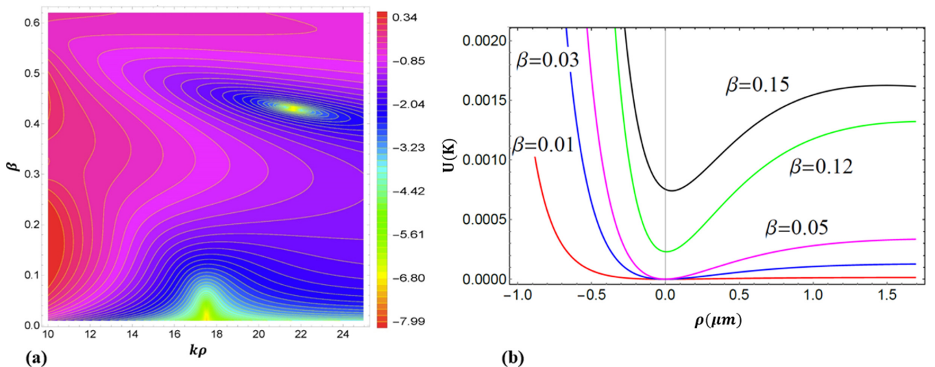
FIG. 12. The dependence of (a) normalized intensity (logarithmic scale) on kx = k\rho and (b) the trap potential on the coordinate y = \rho counted from the center of the trap for different values of \beta for TE_{11,2} resonance. Fixed parameters: kR = 10 and \varepsilon = 3.4975 .
