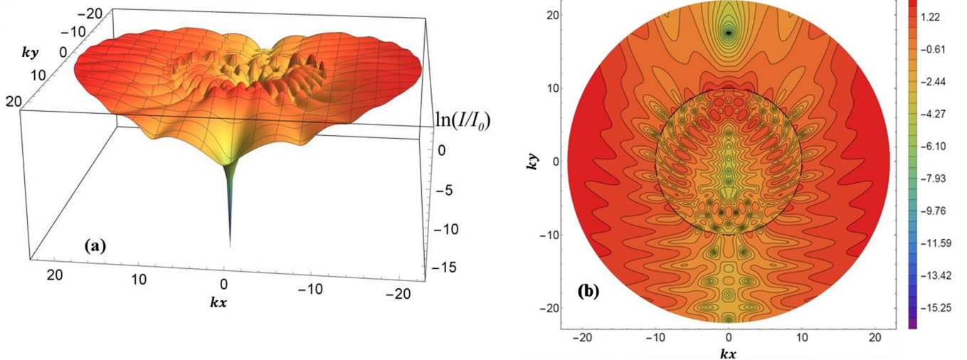
FIG. 4. Normalized intensity I/I_0 on the natural logarithmic scale in the cross section of the cylinder: (a) three-dimensional plot and (b) two-dimensional (2D) color map. Fixed parameters: \beta = 0.01 , kR = 10 , \varepsilon = 3.4975 TE_{11,2} Mie resonance.
