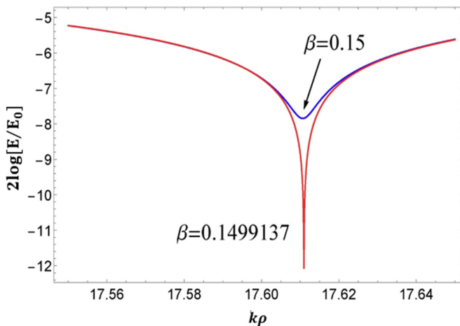
FIG. 17. Spatial distributions of the electric-field magnitude across the trap (logarithmic scale) for initially selected \beta = 0.15 and for optimized \beta = 0.149\,914 . Fixed parameters: kR = 9.3278 and \varepsilon = 3.5 .
