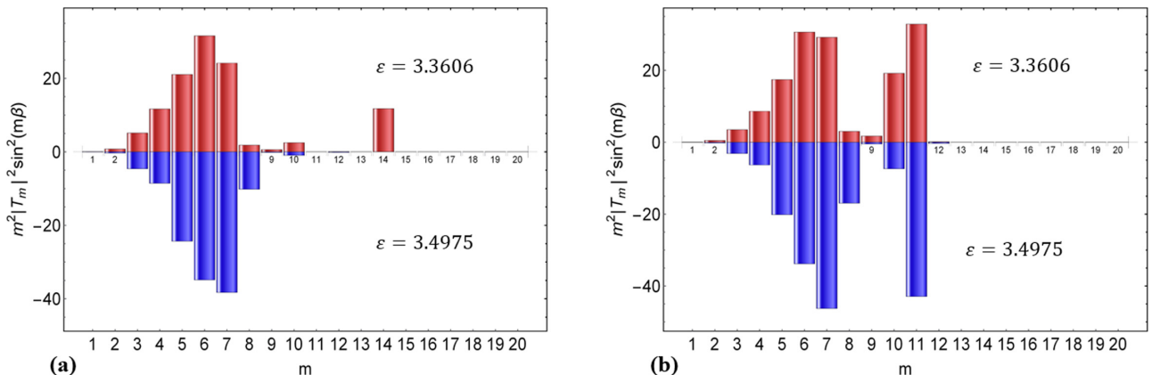
FIG. 2. Modal amplitudes for kR = 10 when (a) \beta = \pi/11 and (b) \beta = \pi/14 .
