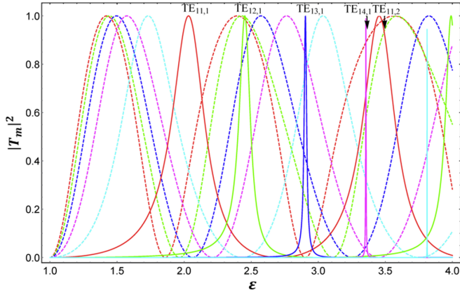
FIG. 3. The dependence of Mie coefficients T_m for m = 6-10 (dashed curves) and m = 11-15 (solid curves) on cylinder permittivity for size parameter kR = 10 . Vertical black arrows correspond to \varepsilon = 3.4975 (near TE_{11,2} Mie resonance, red curve) and to \varepsilon = 3.3606 (near TE_{14,1} Mie resonance, magenta curve).
